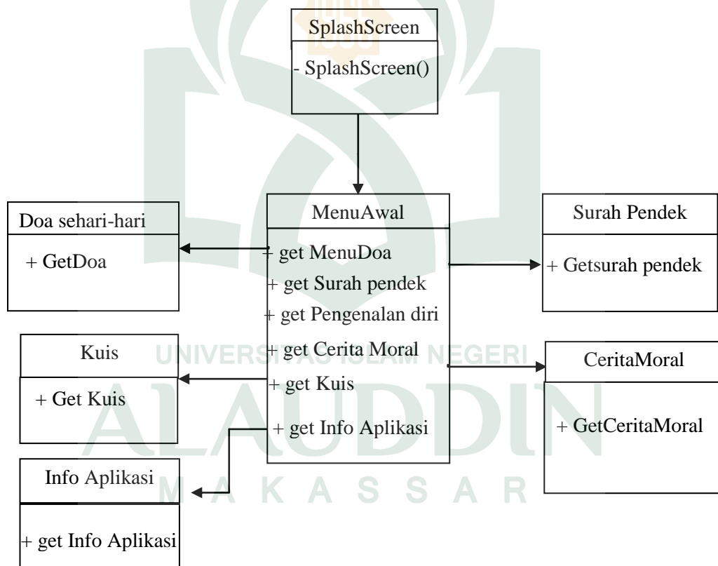
Gambar IV. 4 Class Diagram
