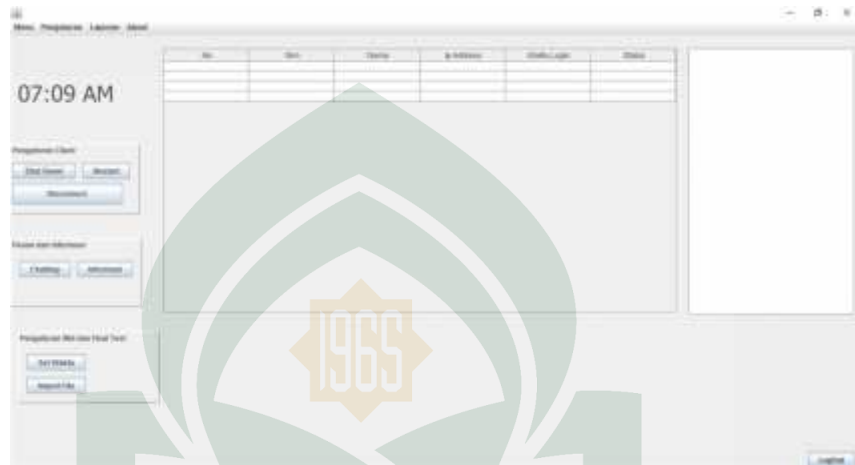
Gambar V.3 Menu Server
