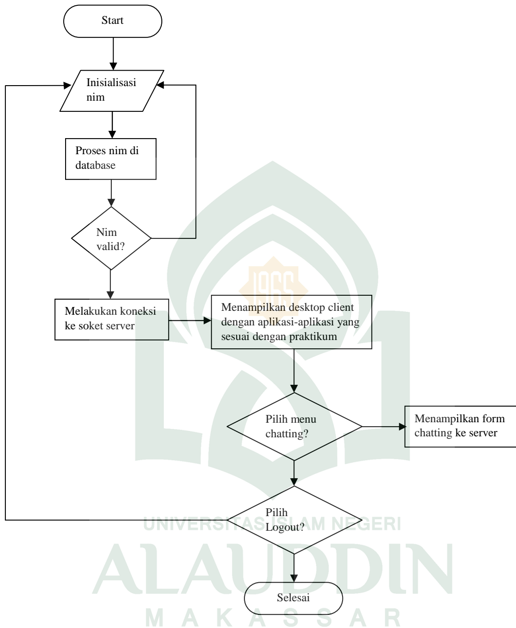
Gambar IV. 17 Flowchart client
