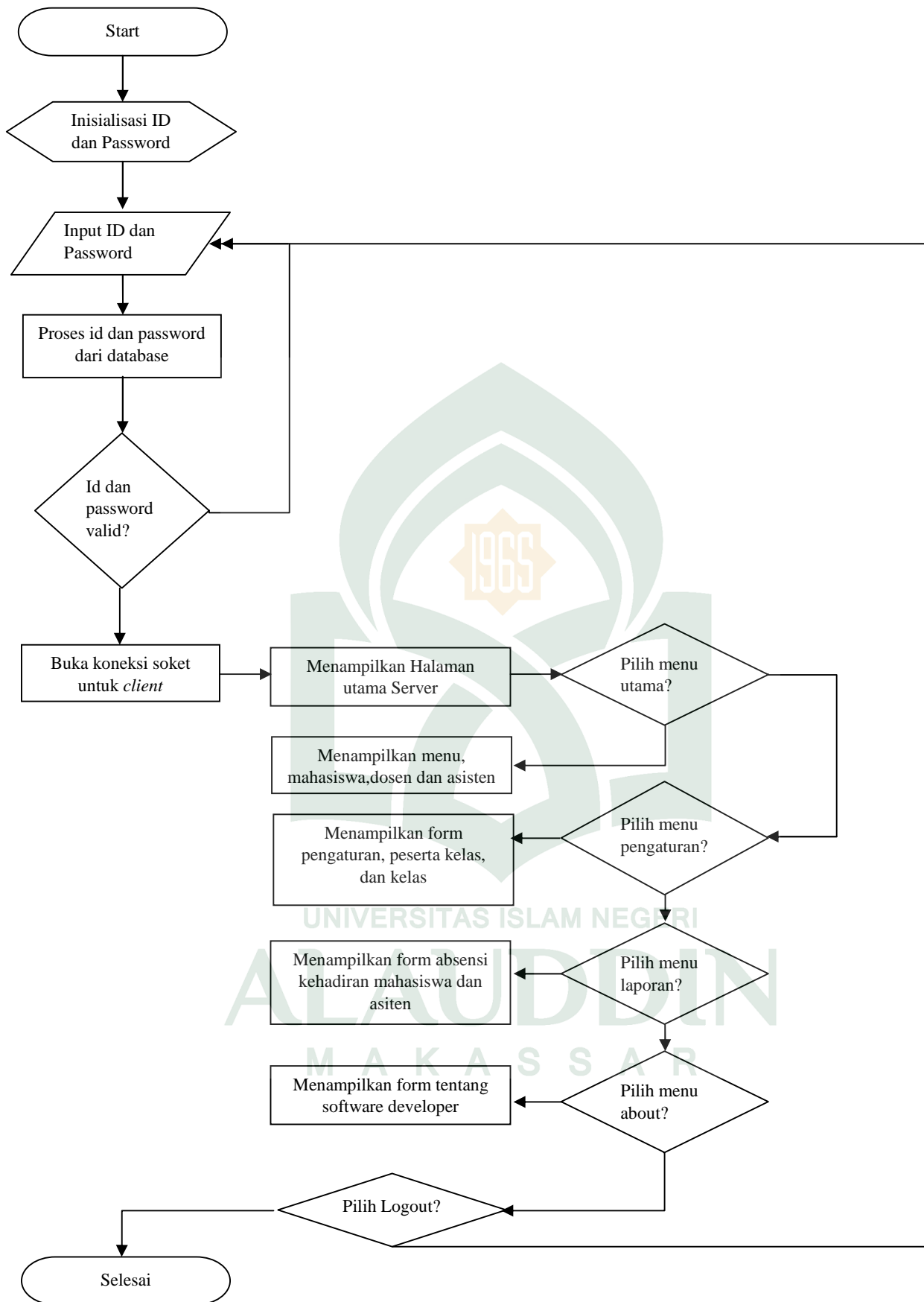
Gambar IV.16 Flowchart Server
