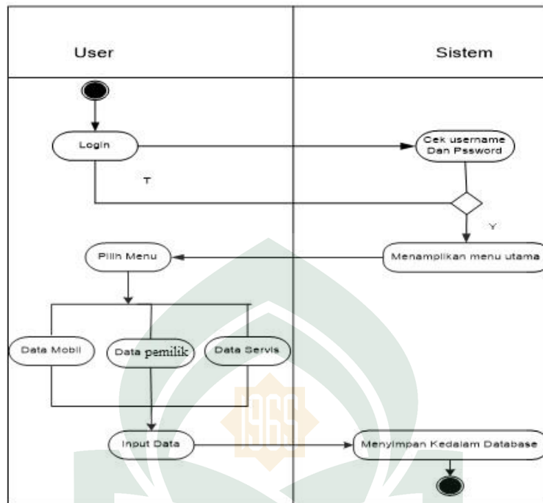
Gambar IV. 4 Activity diagram Admin
