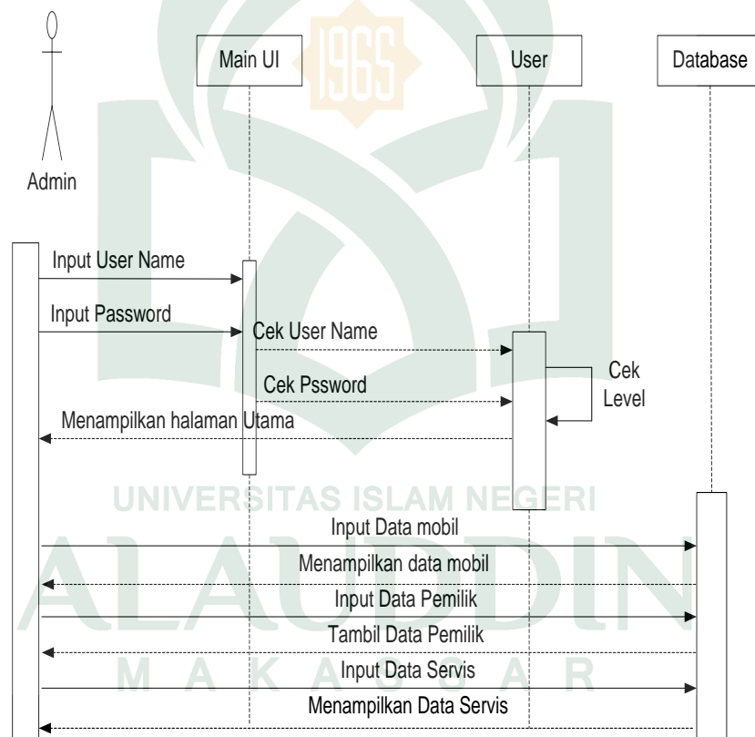
Gambar IV. 6 Sequence Diagram Admin
