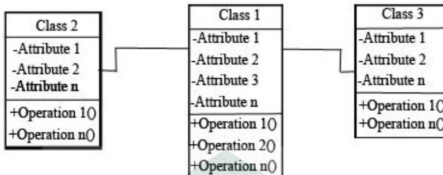
Gambar II. 4 Model Class diagram
