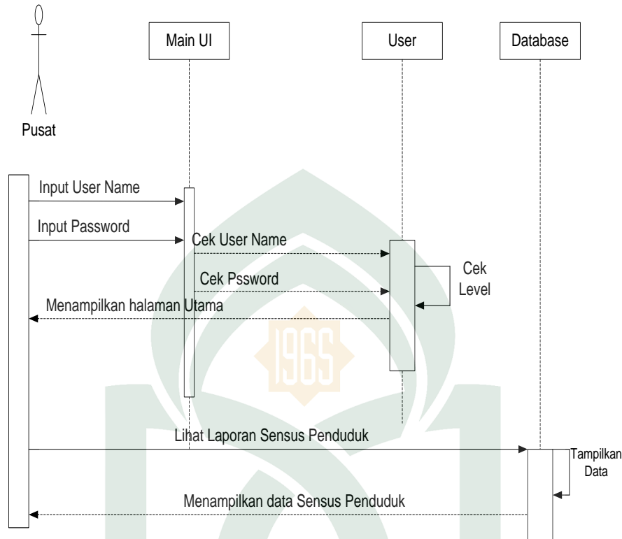
Gambar IV. 7 Sequence Diagram Pusat
