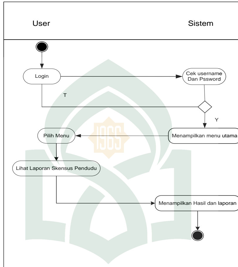
Gambar IV.5 Activity diagram Pusat
