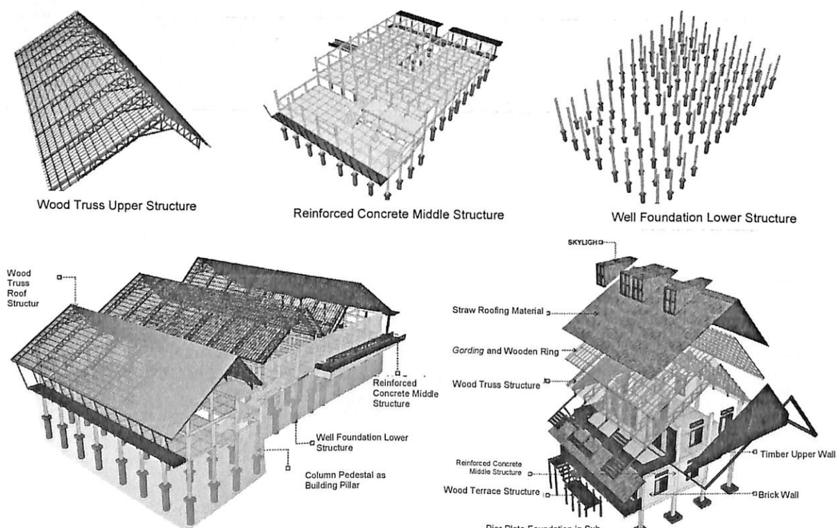
Figure 2. The building structure are roof, middle, and sub structure.
