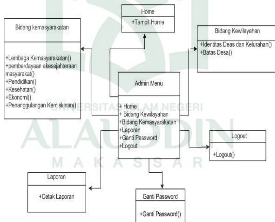
Gambar IV. 4 Class Diagram Admin
