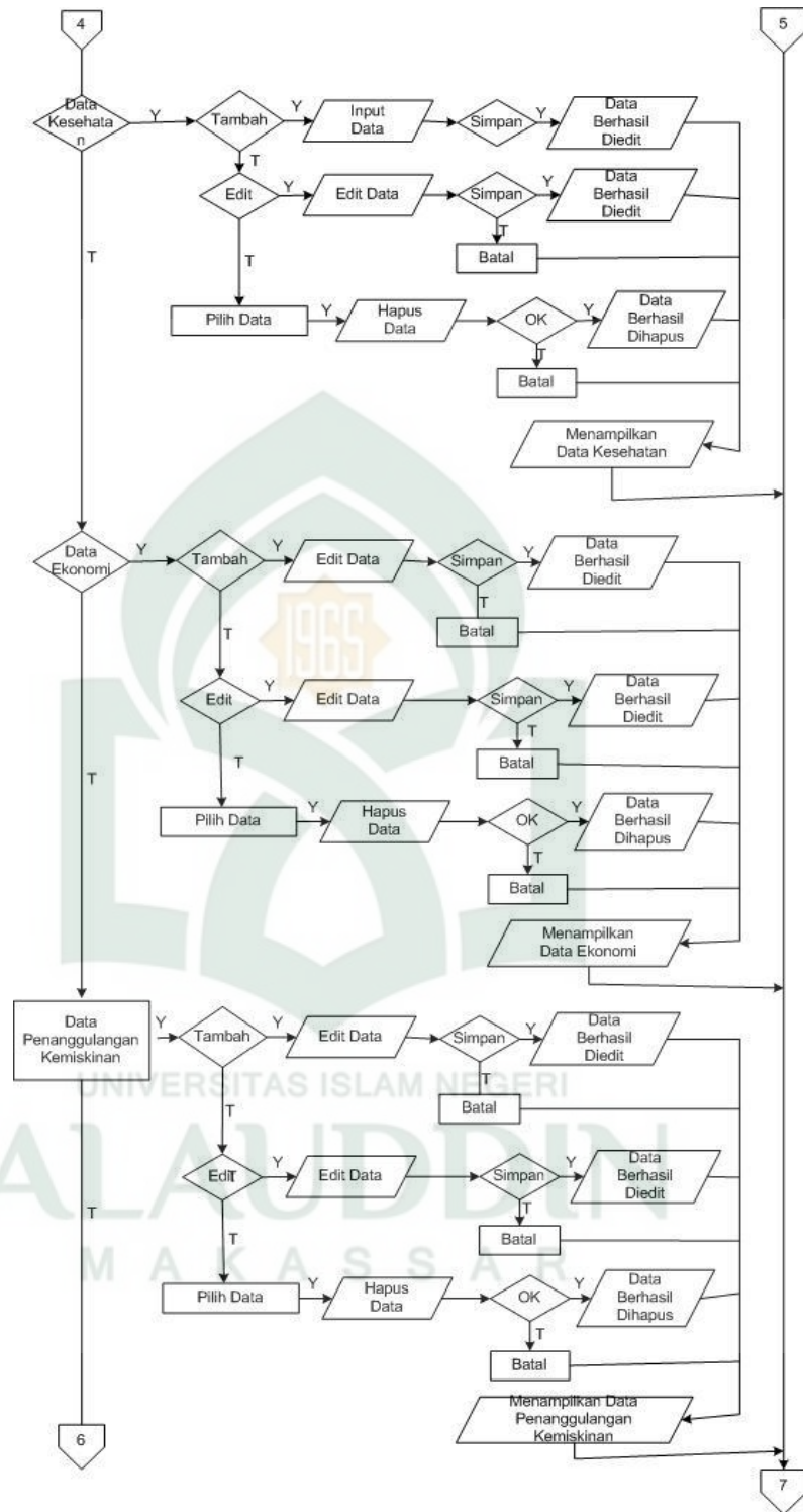
Gambar IV. 22 Flowchart User 3
