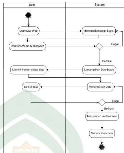
Gambar IV. 12 Activity Diagram Delete Data User
