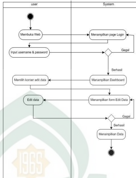
Gambar IV. 11 Activity Diagram Edit Data User
