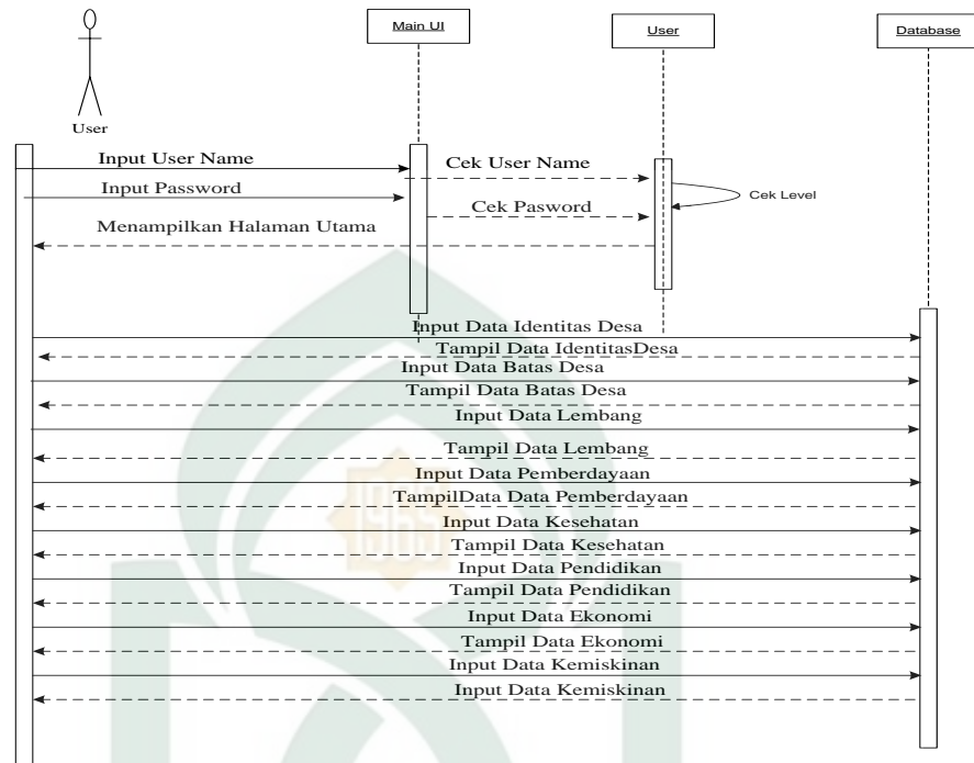
Gambar IV.16 Sequence Diagram Input User
