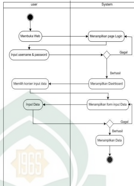
Gambar IV. 10 Activity Diagram Input Data User
