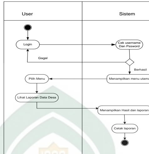
Gambar IV. 13 Activity diagram Laporan Admin
