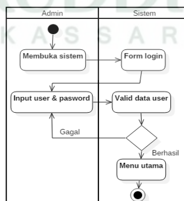
Gambar IV.6 Activity diagram Login Admin
