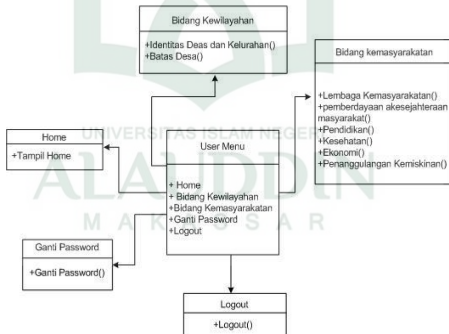
Gambar IV. 5 Class Diagram User
