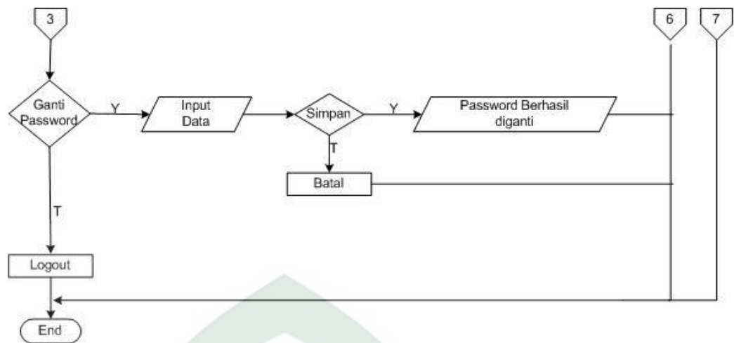
Gambar IV 23 Flowchart User 4
