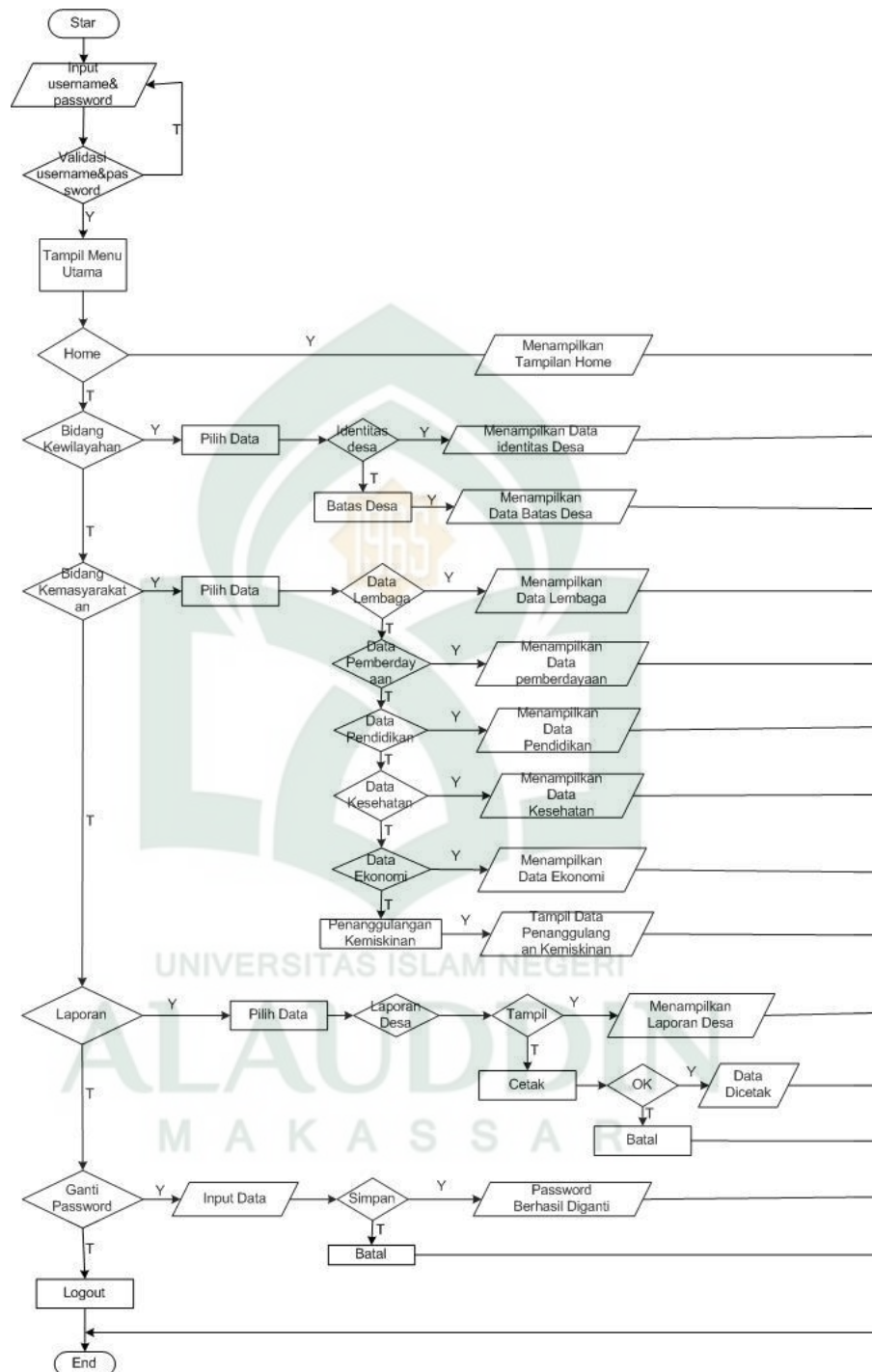
Gambar IV. 19 Flowchart Admin
