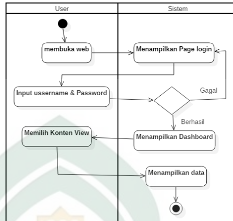
Gambar IV. 9 Activity Diagram View Data User
