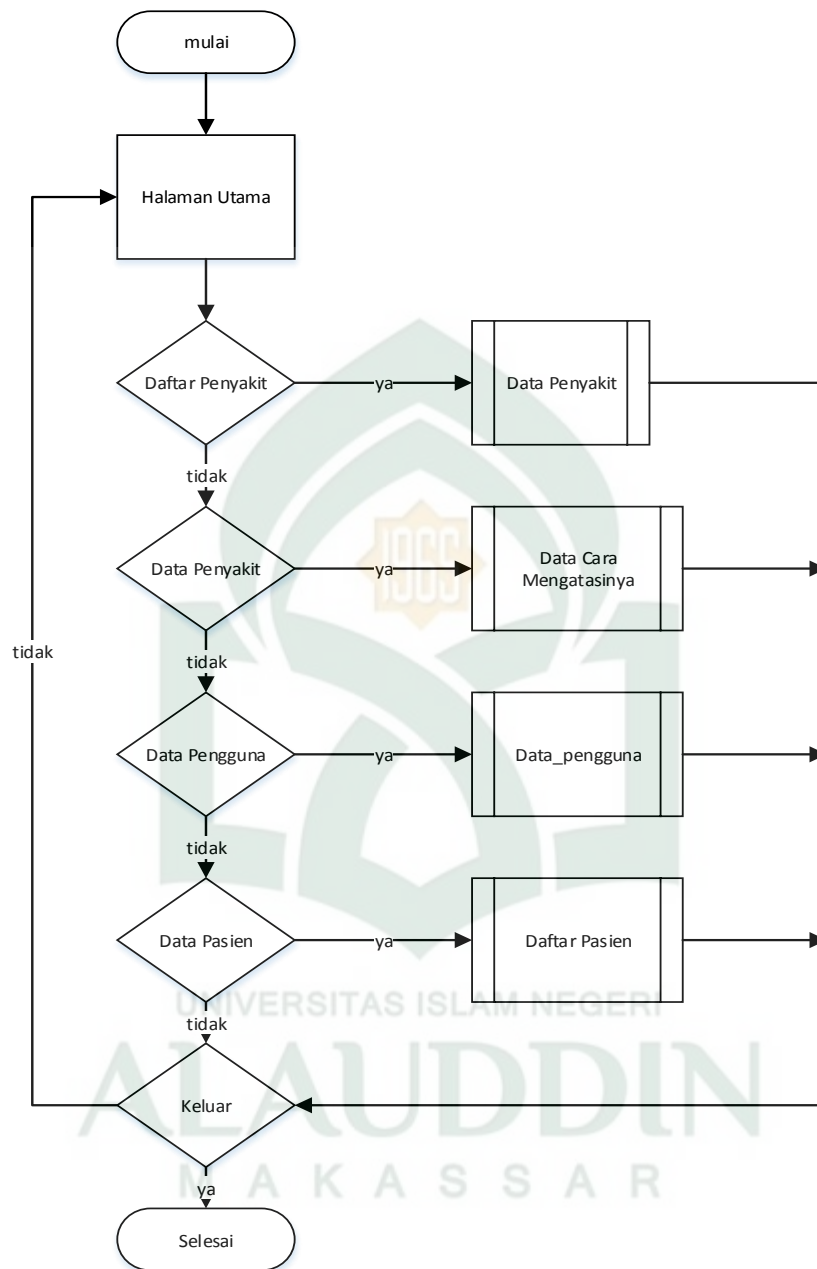
Gambar IV-9. Flowchart Menu Admin (Alur Program)
