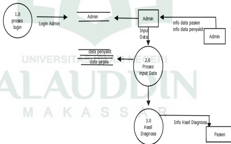
Gambar IV-4. Data Flow Diagram level 1 proses 1
