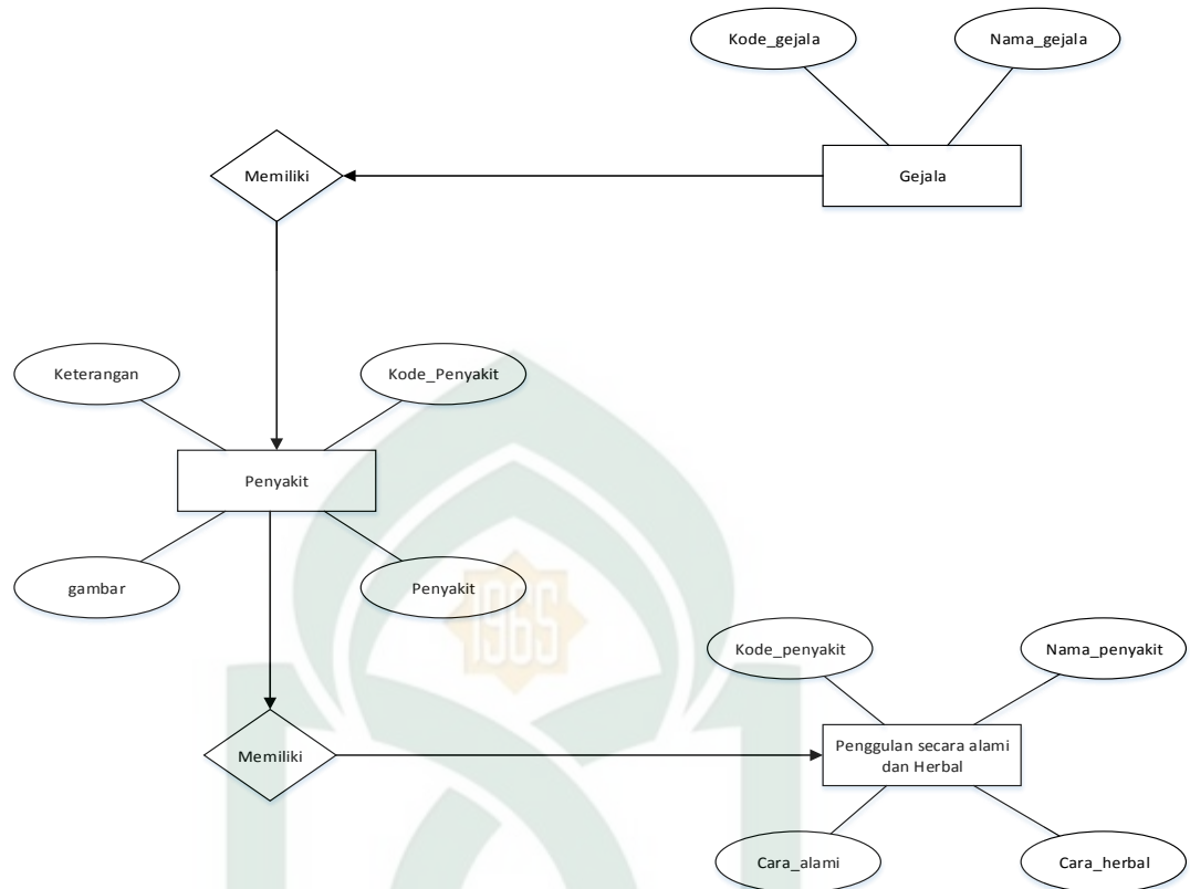
Gambar IV-7. Entity Relationship Diagram
