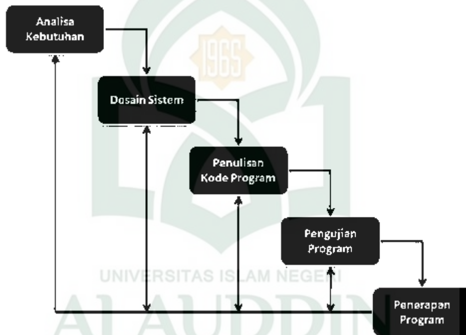
Gambar III.1. Metode Waterfall
