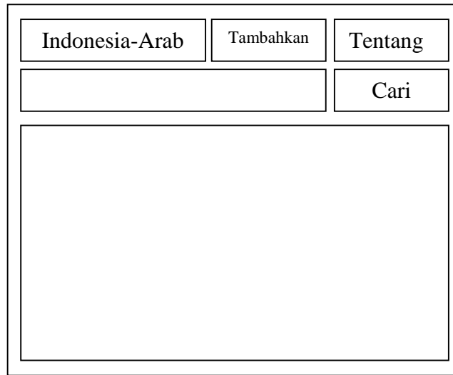
Gambar IV.9 Splash Screen
