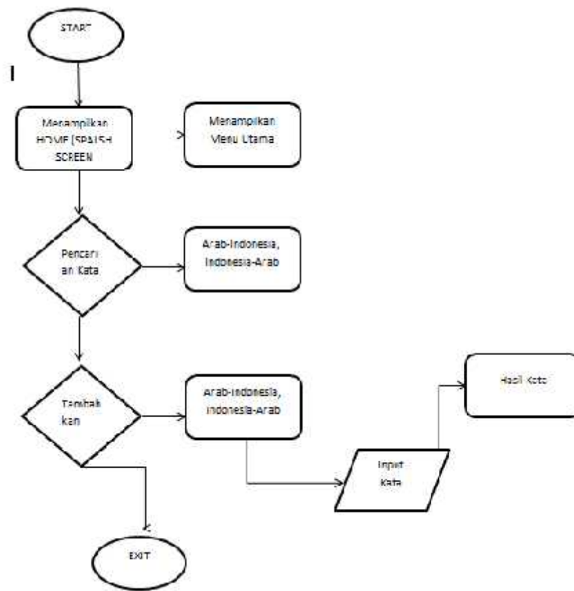
Gambar IV.8 Flowchart
