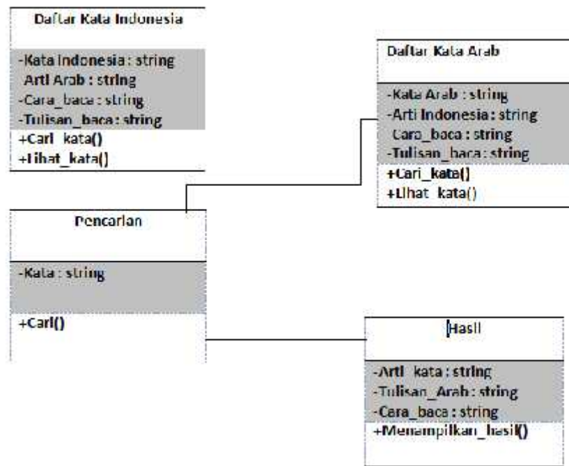
Gambar IV.5 Class Diagram
