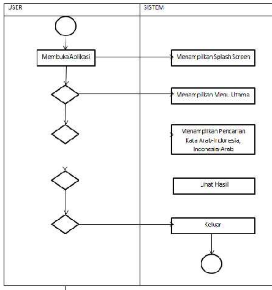
Gambar IV.7 Activity Diagram
