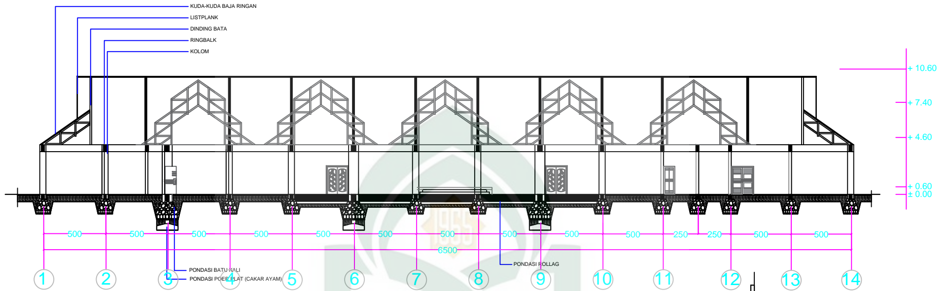
POTONGAN X-X SKALA = 1:300
