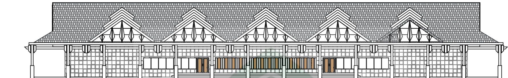
TAMPAK DEPAN (E) SKALA = 1:300
