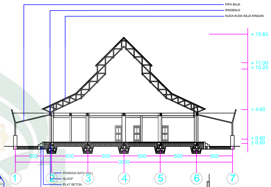
POTONGAN X-X SKALA = 1:300
