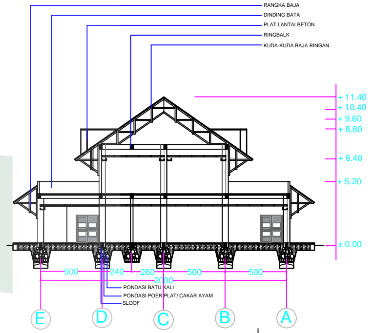
POTONGAN Y-Y SKALA = 1:300
