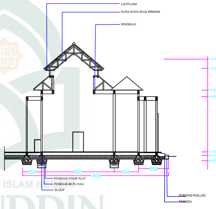
POTONGAN Y-Y SKALA = 1:300
