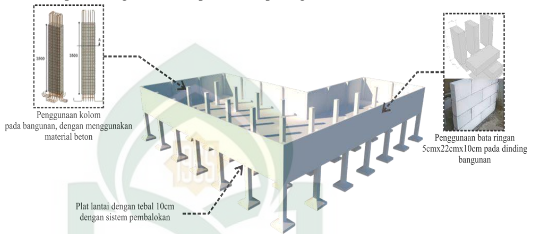
Gambar III.42 Middle Structure (Sumber : Olah Desain, 2018)
