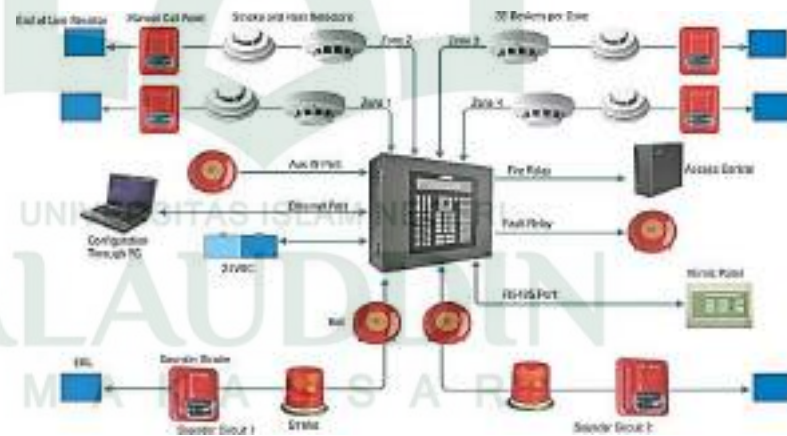
Gambar III.37 Sistem Kerja Fire Alarm
