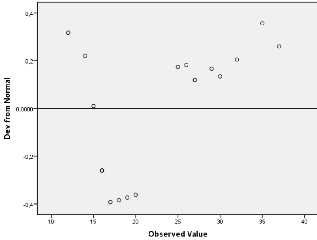
Detrended Normal Q-Q Plot of VAR00001
