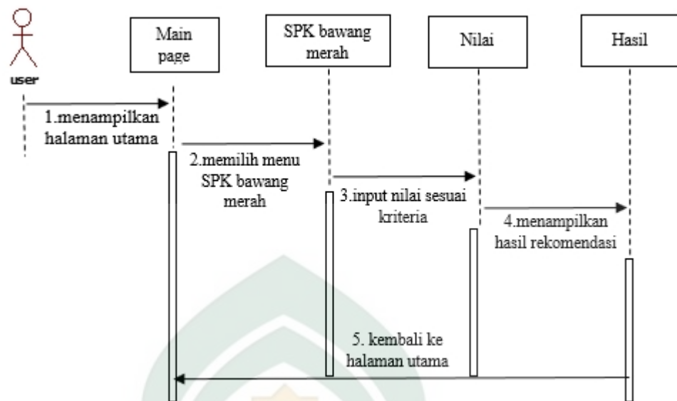
Gambar IV.9 Sequence diagram user
