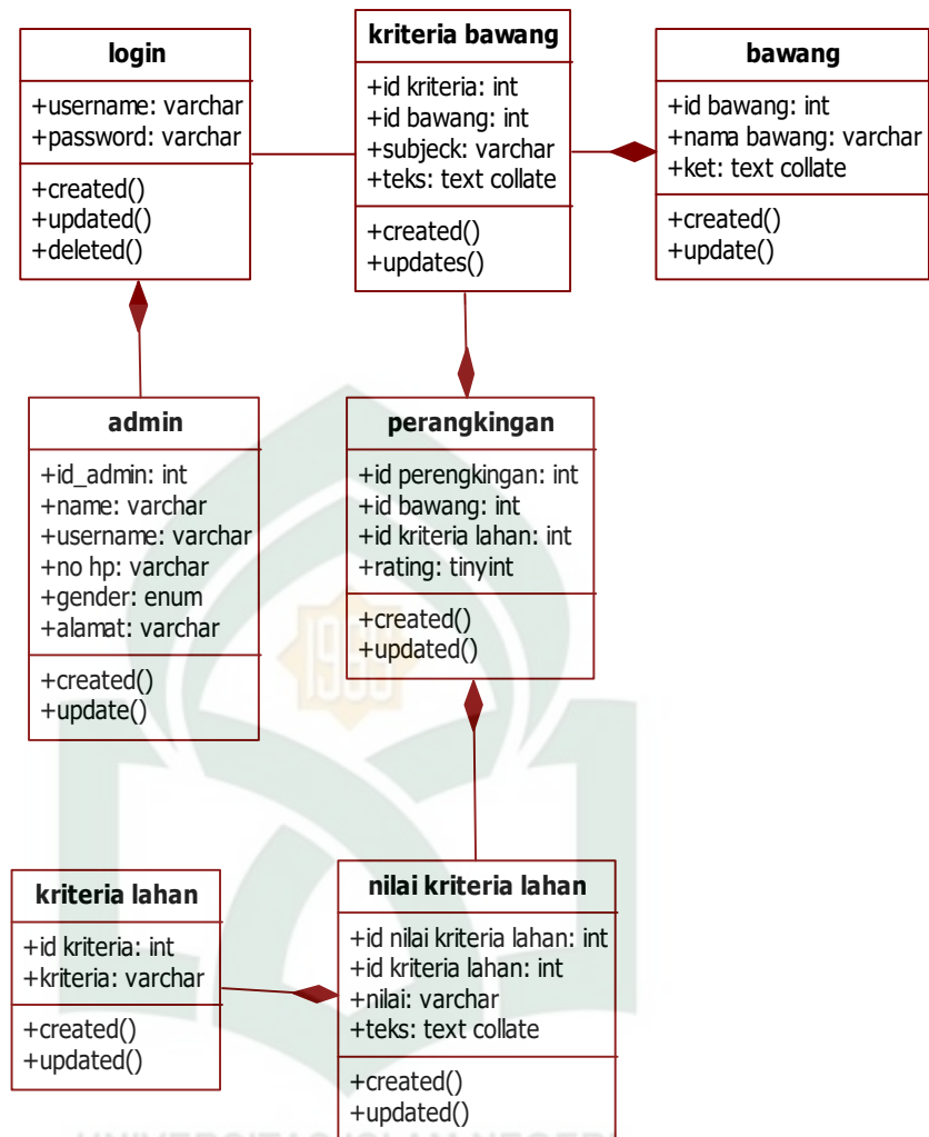
Gambar IV.8 class diagram
