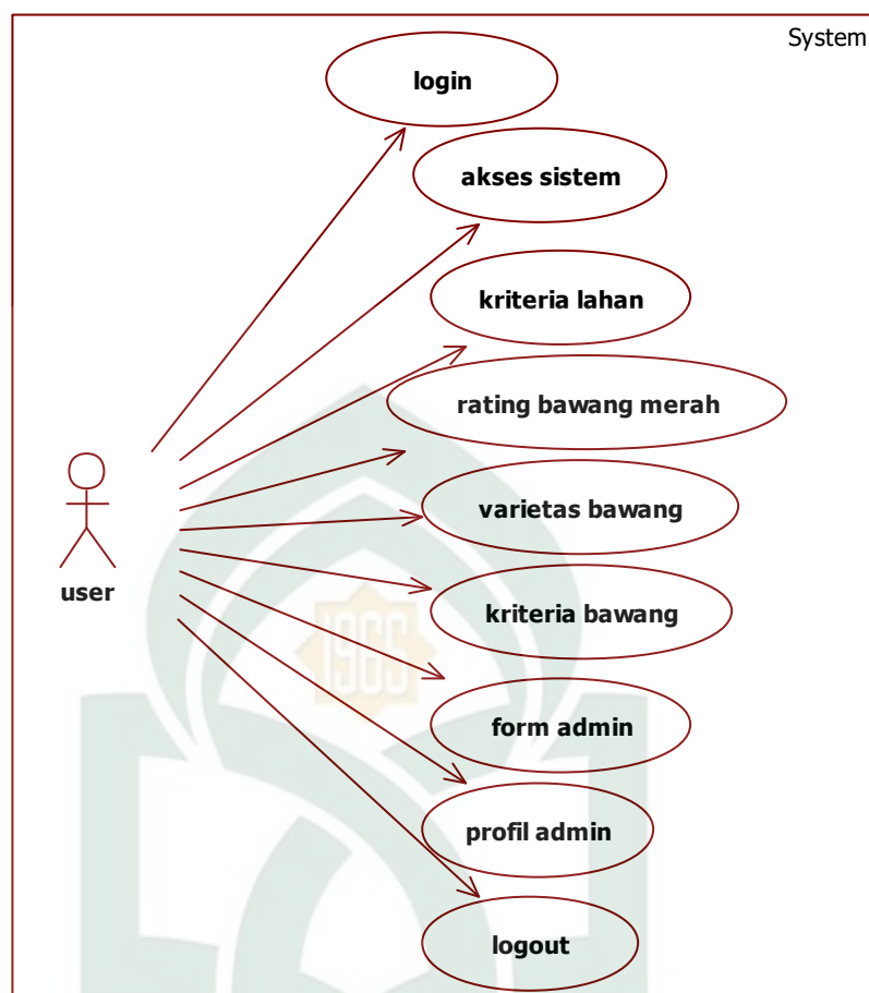
Gambar IV.7 use case diagram admin
