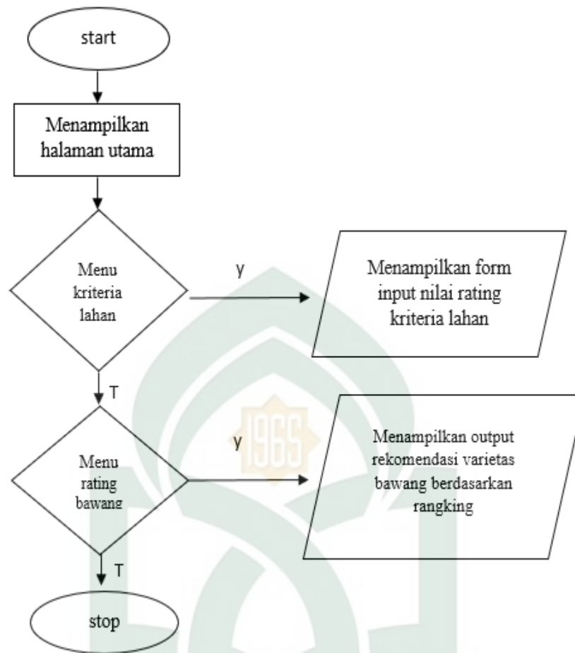
Gambar IV.12 Flowchart
