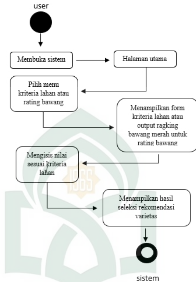
Gambar IV.10 Activity diagram
