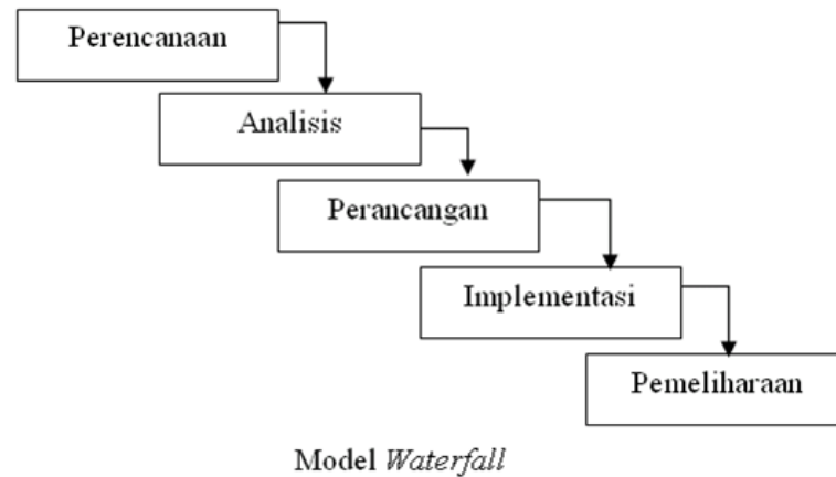
Gambar III.1. Model Waterfall
