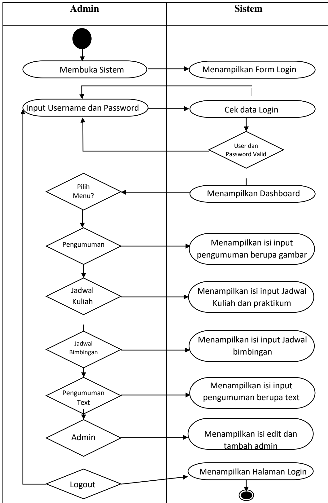
Gambar IV.10 Diagram Activity
