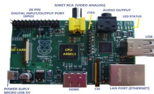
Gambar II.2. Raspberry pi board
