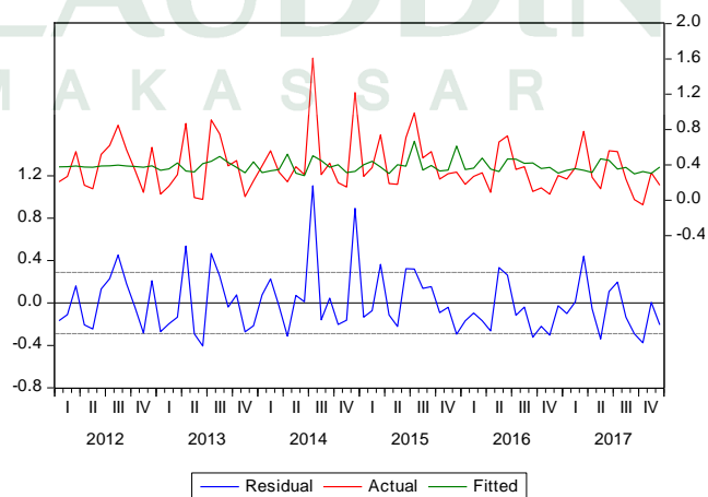
Gambar 4.9: Grafik uji residual model ARMA(0,4)
