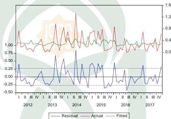
Gambar 4.24: Grafik uji residual model ARMA(0,6)
