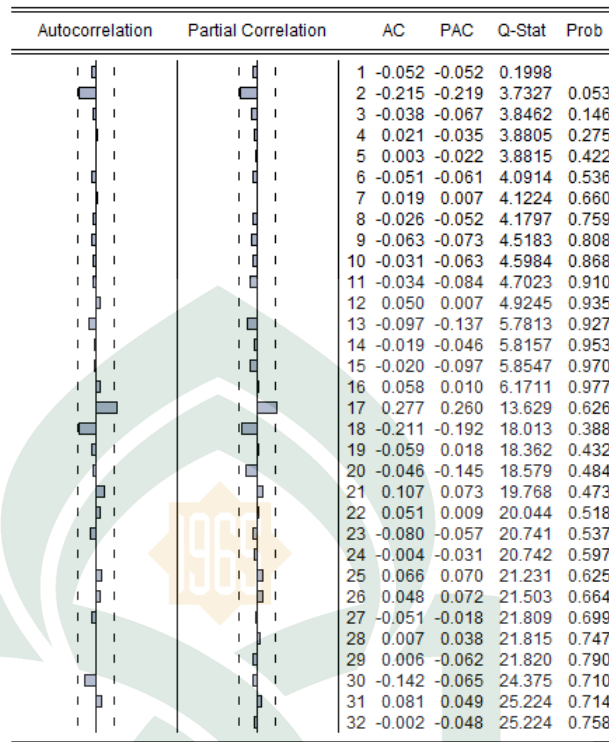
Gambar 4.35: Collegram residual model ARMA(0,1)
