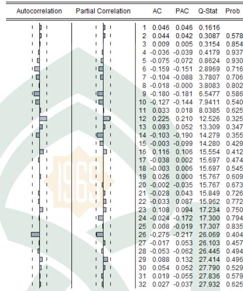
Gambar 5.15: Collogram residual model ARMA(3,2)
