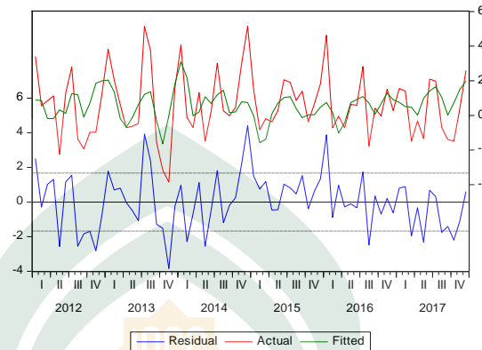
Gambar 4.4: grafik uji residual model ARMA(3,2)
