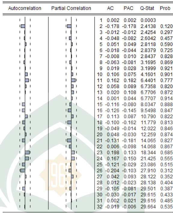
Gambar 4.25: Collegram residual model ARMA(0,6)
