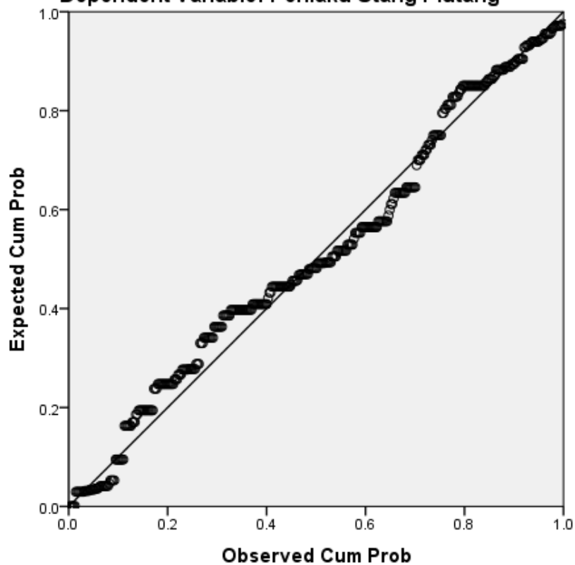
Normal P-P Plot of Regression Standardized Residual Dependent Variable: Perilaku Utang Piutang
