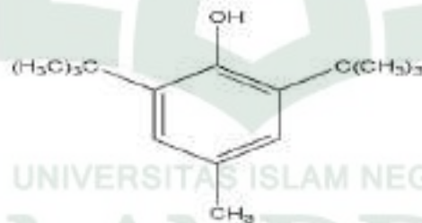
Gambar 8. Rumus Struktur Butylated Hydroxytoluene
