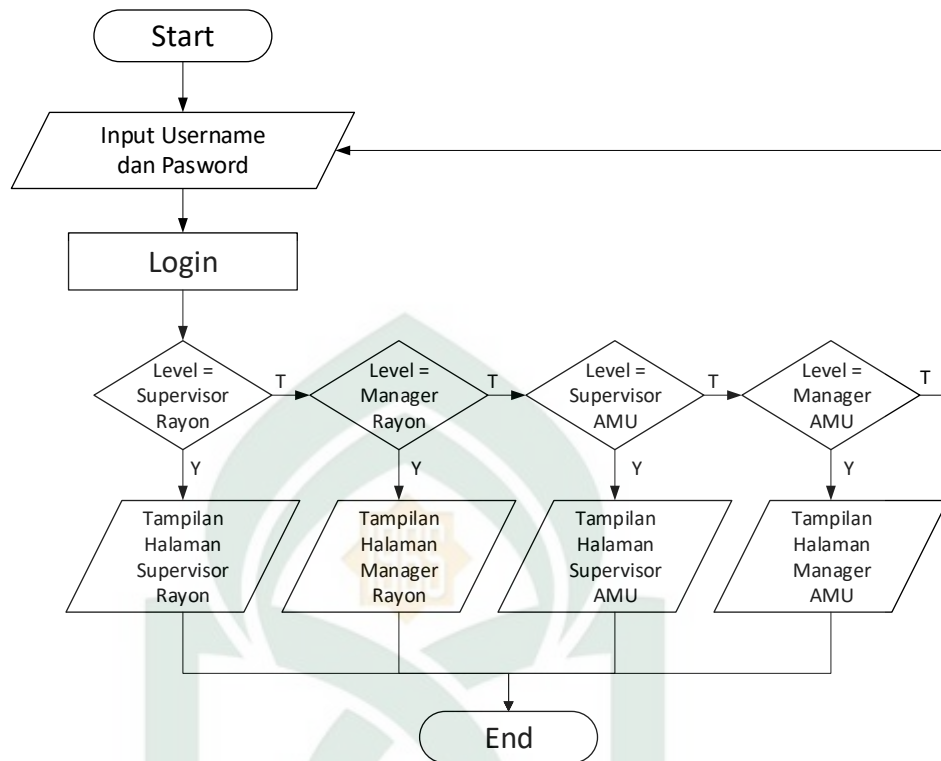
Gambar IV.7. Flowchart
