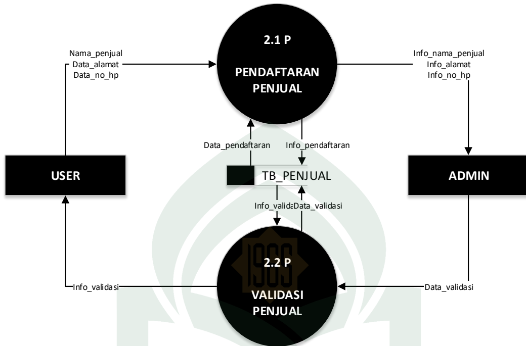
Gambar IV.8. DFD level 2 proses 2
