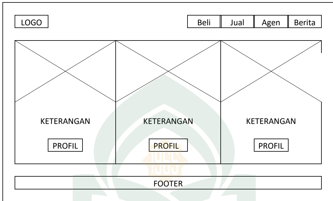
Gambar IV.17. Halaman Agen
