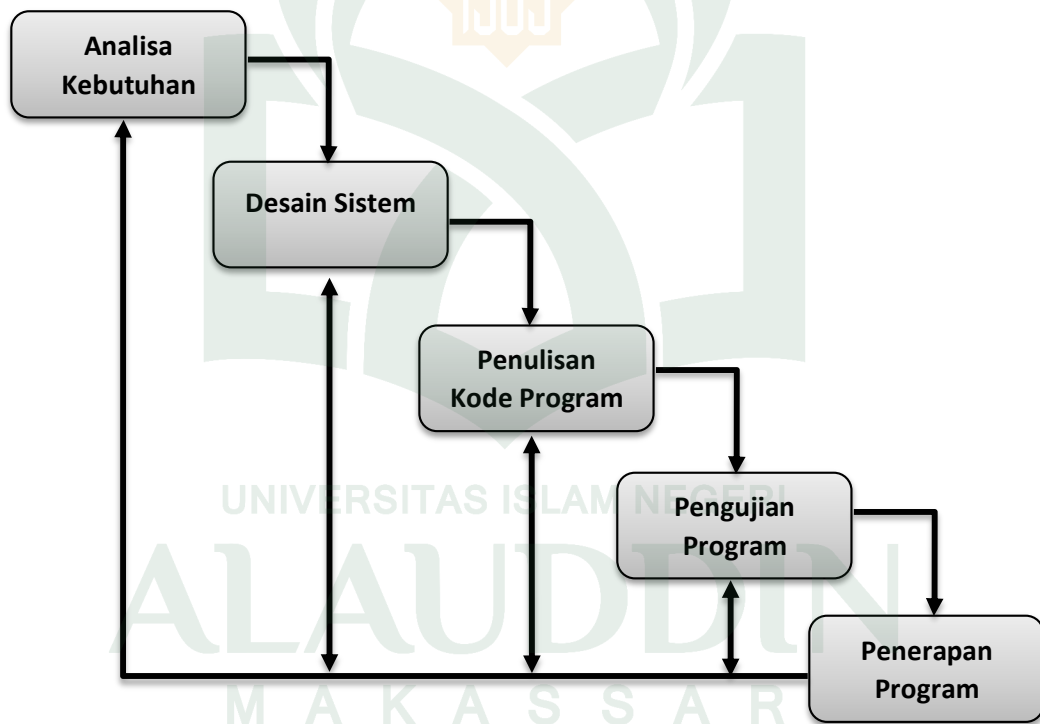
Gambar III.3. Model Waterfall
