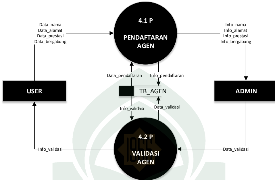
Diagram IV.10. DFD level 2 proses 4
