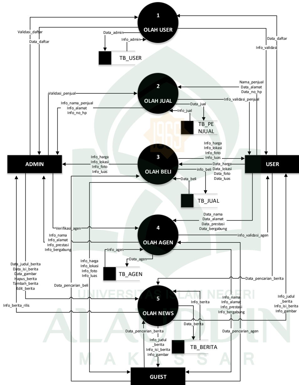
Diagram IV.6. Data flow diagram level 1
