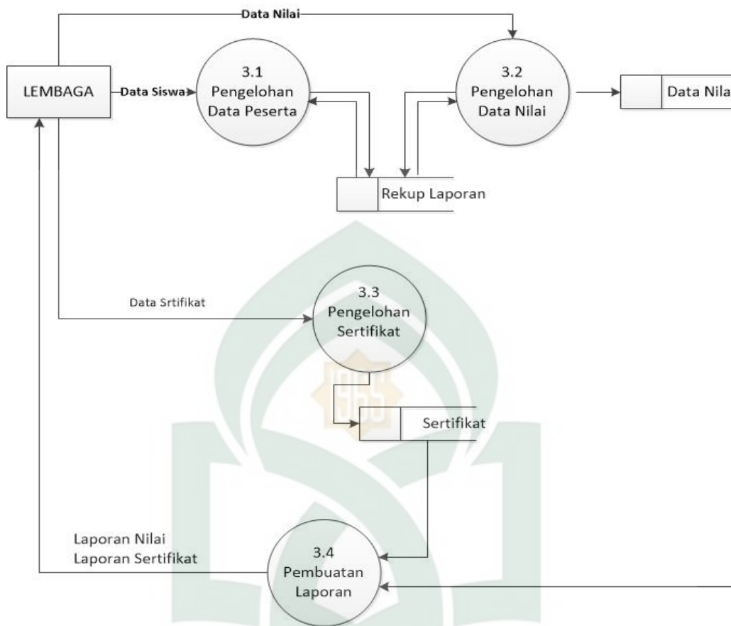
Gambar IV. 5. Data Flow Digram Level 2 Proses 1
