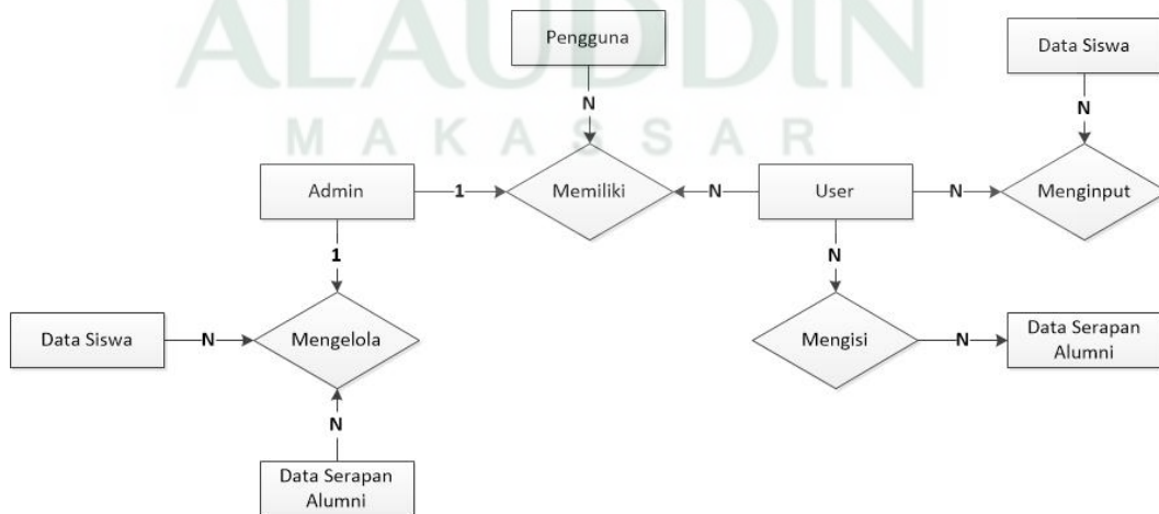
Gambar IV. 6. Entity Relationship Diagram
