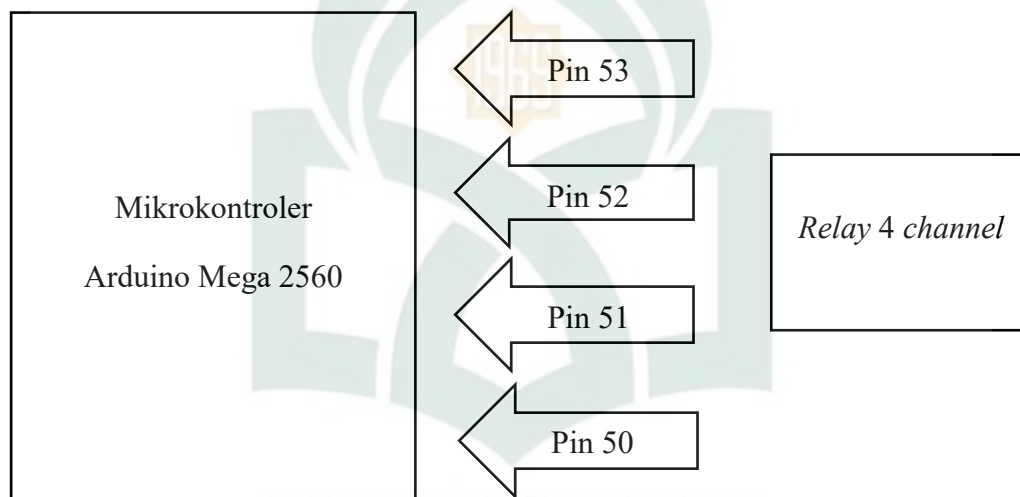
Gambar IV.9. Ilustrasi Relay 4 Channel
