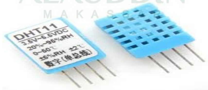
Gambar II. 4. Sensor DHT11 ( Sumber: www.bdspeedytech.com )
