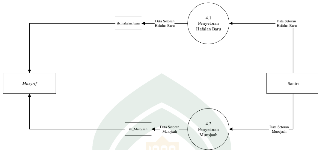
Gambar IV.6 DFD Level 2 Proses 4
