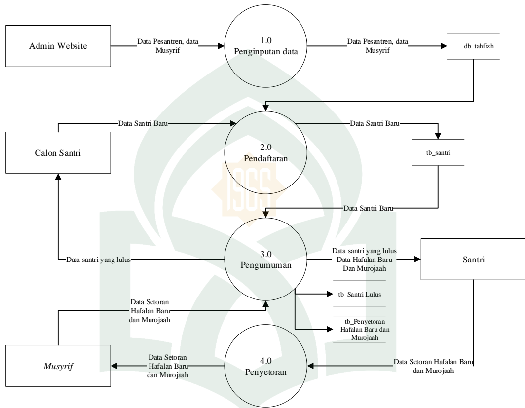
Gambar IV.5 DFD Level 1
