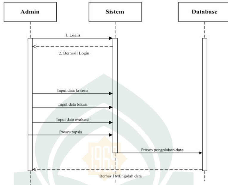
Gambar IV.4 Sequence Diagram
