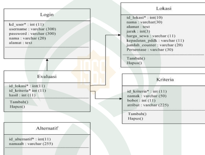
Gambar IV. 3 Class Diagram
