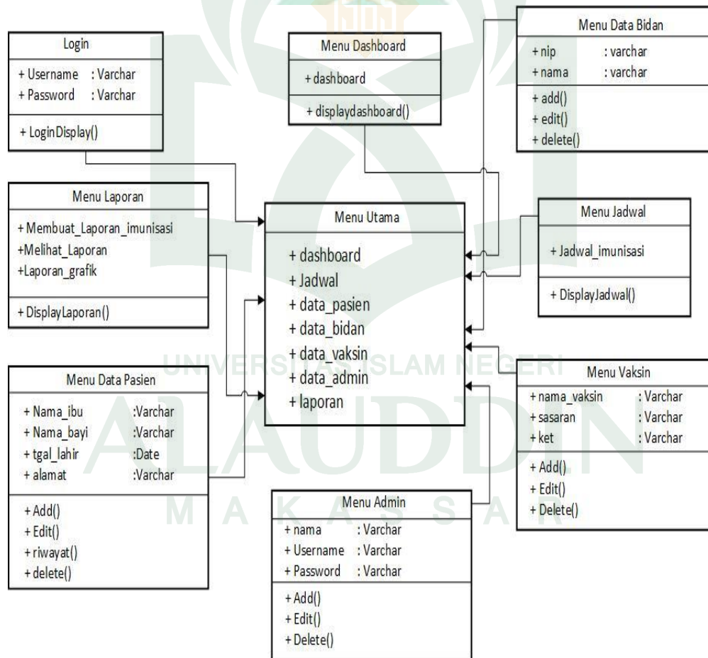
Gambar.IV 3 Class Diagram
