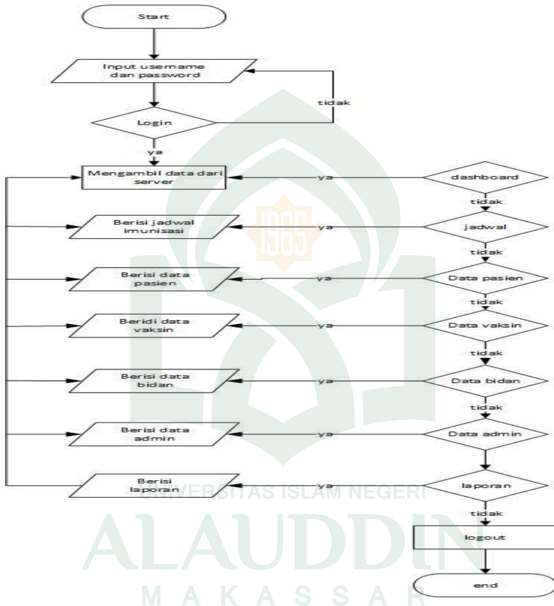
Gambar.IV 16 Flowchart Sistem
