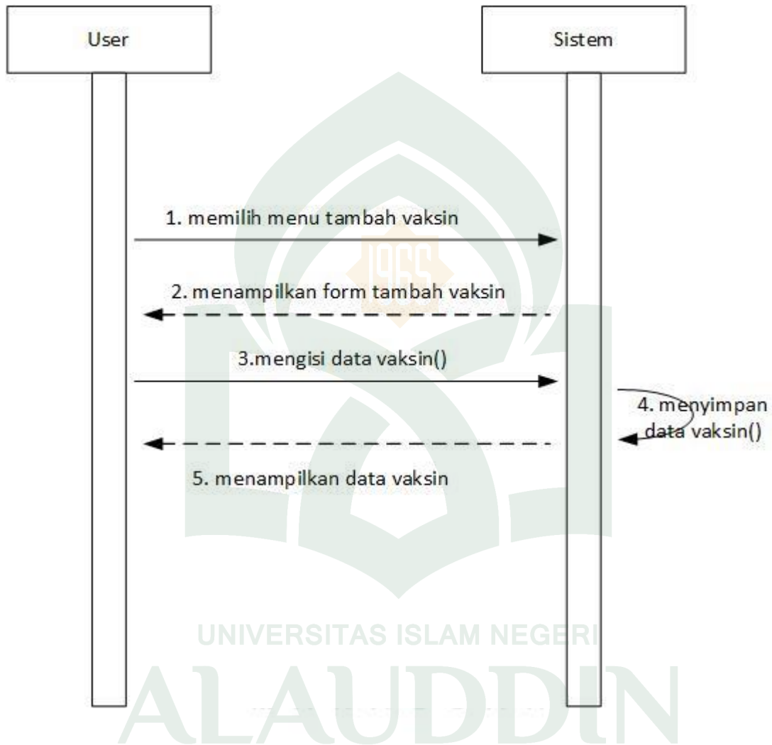
Gambar.IV 10 Sequence Sub Menu Tambah Vaksin
