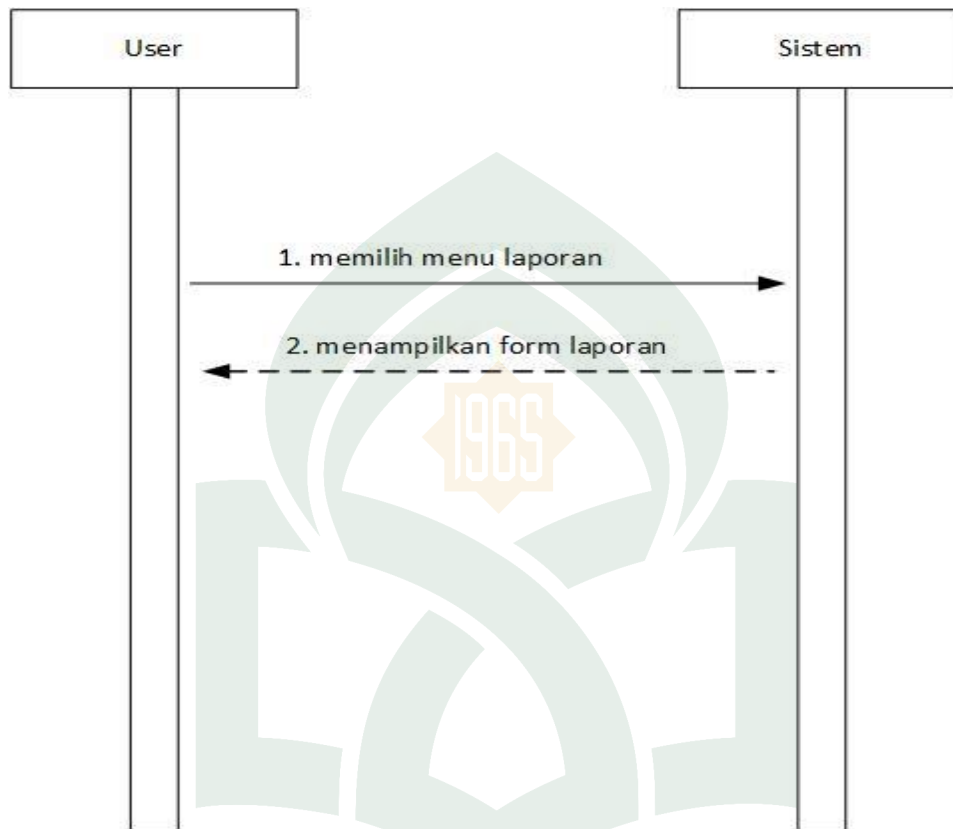
Gambar.IV 6 Sequence Menu Laporan
