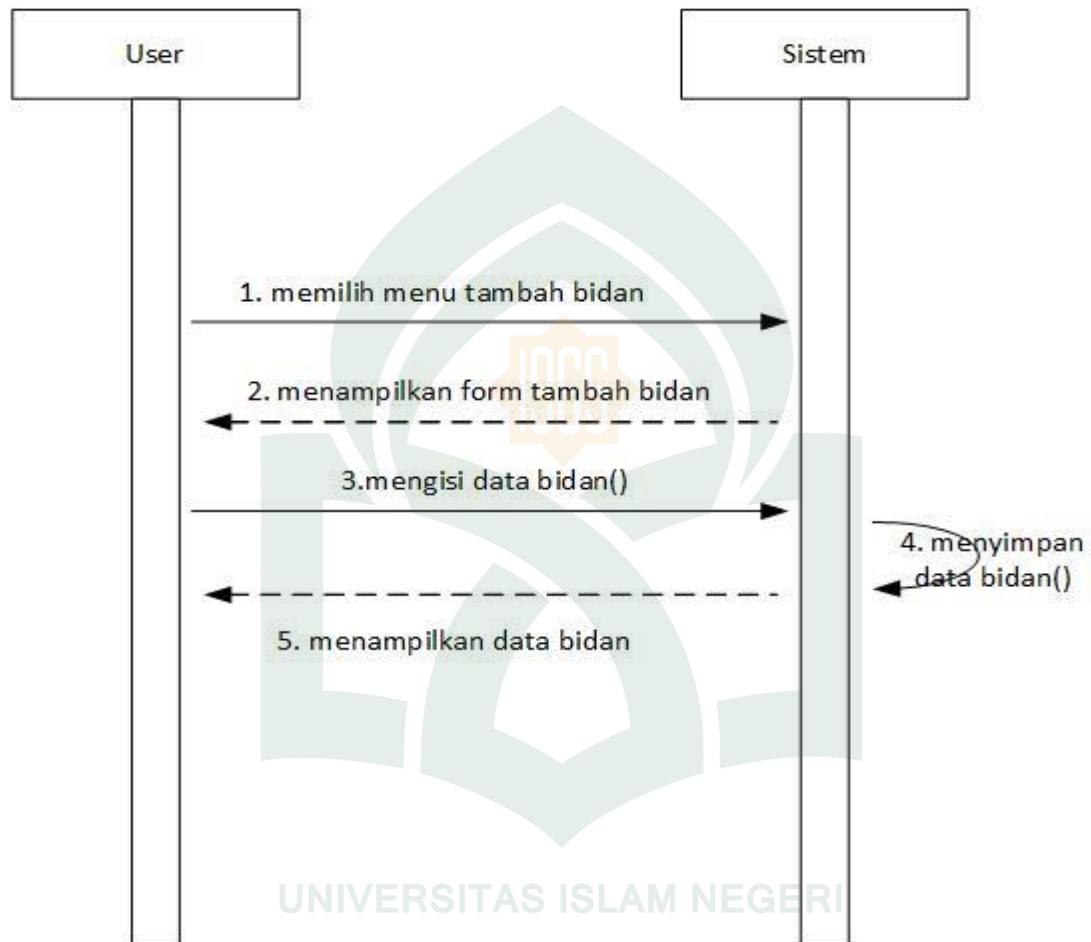
Gambar.IV 12 Sequence Sub Menu Tambah Bidan
