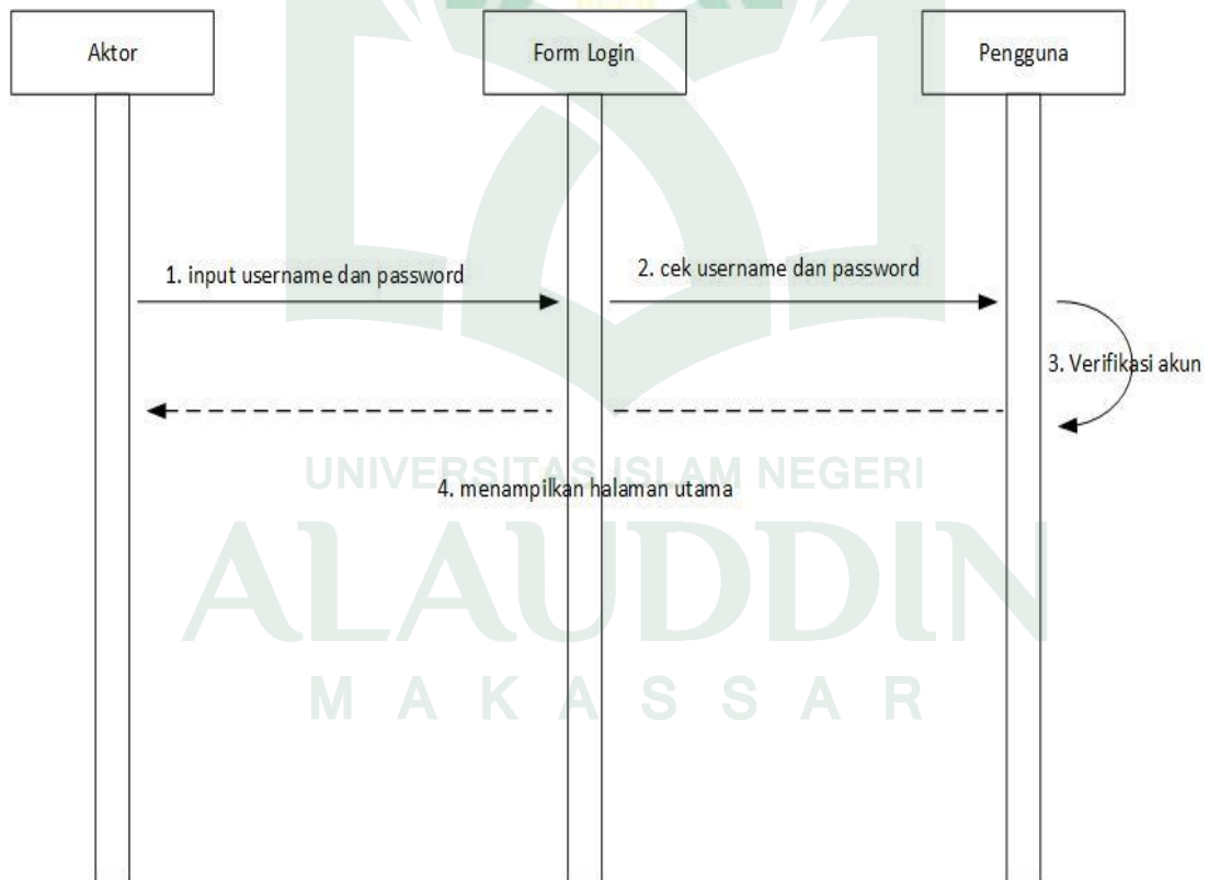
Gambar.IV 4 Sequence Menu Login
