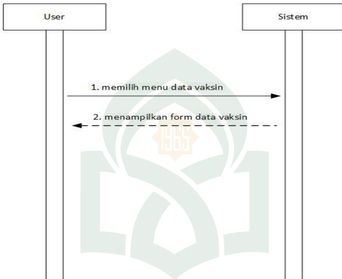
Gambar.IV 11 Sequence Sub Menu Data Vaksin
