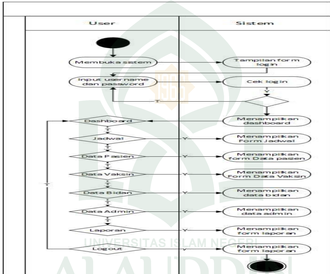
Gambar.IV 14 Activity Diagram
