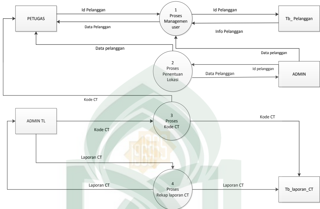
Gambar IV.7 Data Flow Diagram level 1
