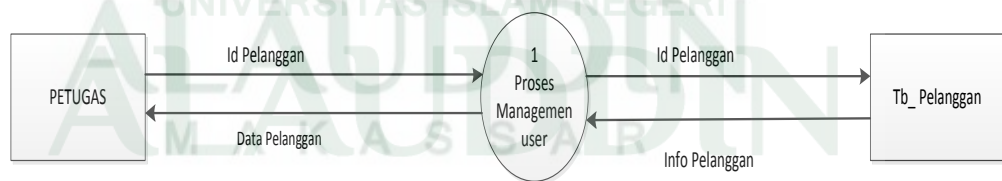
Gambar IV.8 Data Flow Diagram Level 2 proses I
