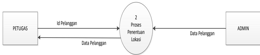
Gambar IV.9 Data Flow Diagram Level 2 proses II
