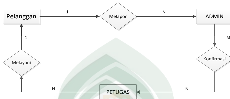
Gambar IV.12 Diagram ERD
