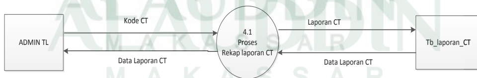
Gambar IV.11 Data Flow diagram Level 2 proses IV
