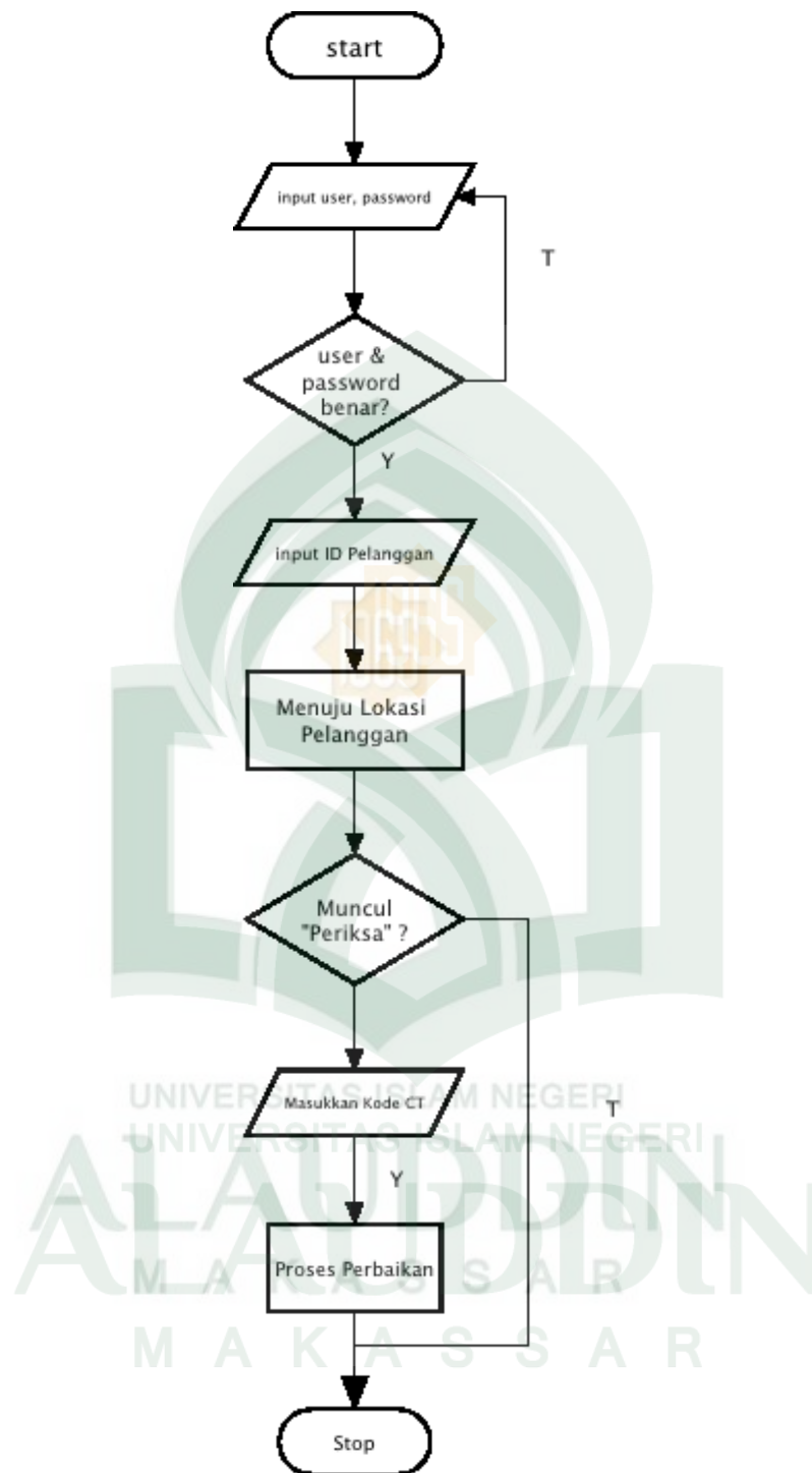
Gambar IV.3 Flowchart User (Petugas Yantek)
