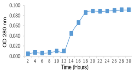
Figure 1. Growth curve of Bacillus coagulans
