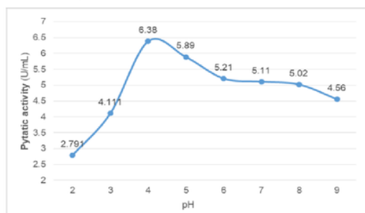
Figure 3. Phytase activity of Bacillus coagulans on the pH variation
