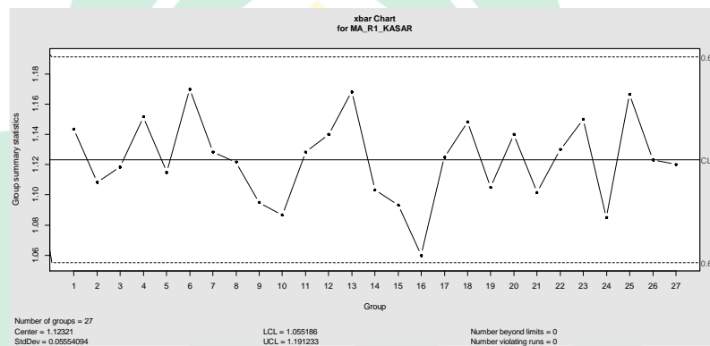
Gambar 4.11 Peta Kendali Mean Aperture Grain Size R1 Kasar Revisi 2
