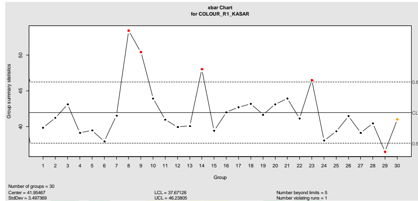
Gambar 4.7 Peta Kendali Colour R1 Kasar
