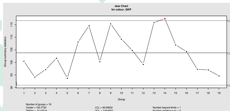
Gambar 4.18 Peta Kendali Colour GKP Revisi 2
