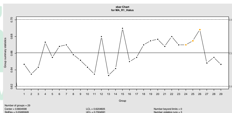
Gambar 4.15 Peta Kendali Mean Aperture Grain Size R1 Halus Revisi
