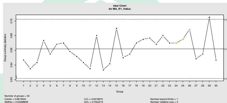
Gambar 4.14 Peta Kendali Mean Aperture Grain Size R1 halus
