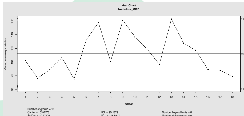
Gambar 4.19 Peta Kendali Colour GKP Revisi 3
