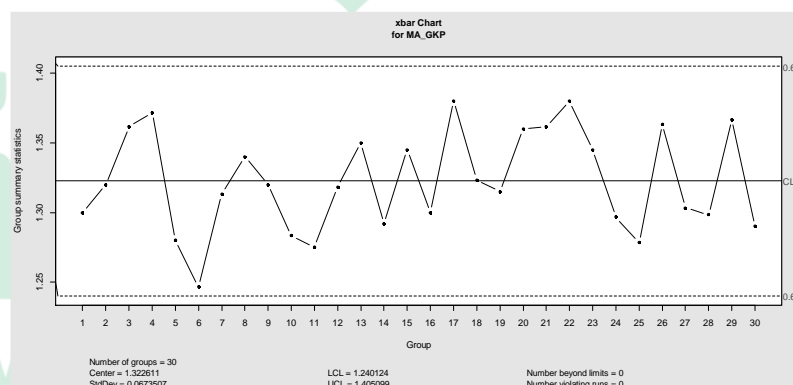
Gambar 4.20 Peta kendali Mean Apperture Grain Size GKP
