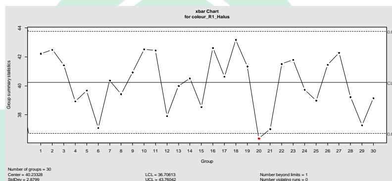
Gambar 4.12 Peta Kendali colour R1 Halus
