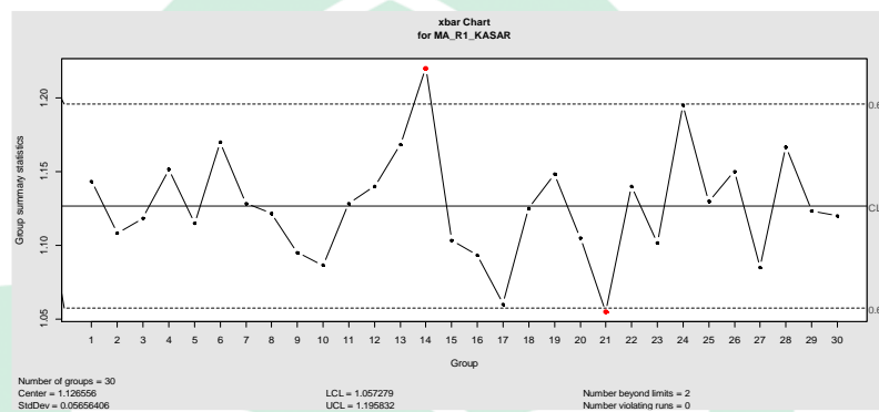
Gambar 4.9 Peta Kendali Mean Apperture Grain Size R1 Kasar
