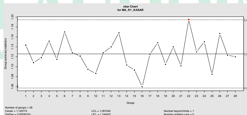
Gambar 4.10 Peta kendali Mean Apperture Grain Size R1 Kasar Revisi 1
