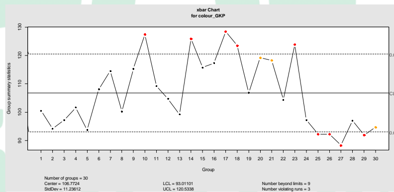
Gambar 4.16 Peta Kendali Colour GKP
