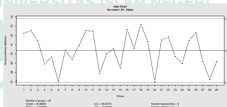
Gambar 4.13 Peta Kendali colour R1 Halus Revisi
