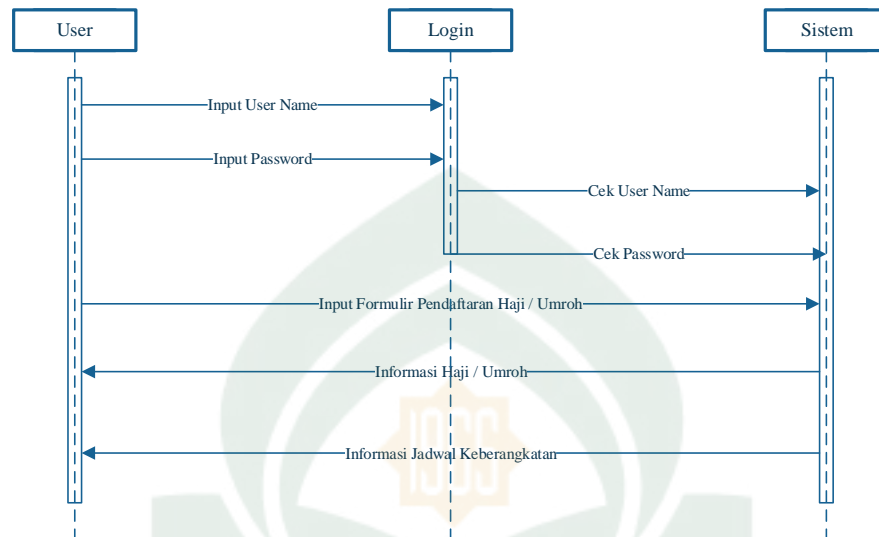
Gambar IV.6 Sequence Diagram
