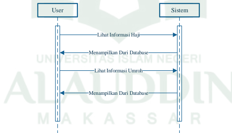
Gambar IV.7 Sequence Diagram
