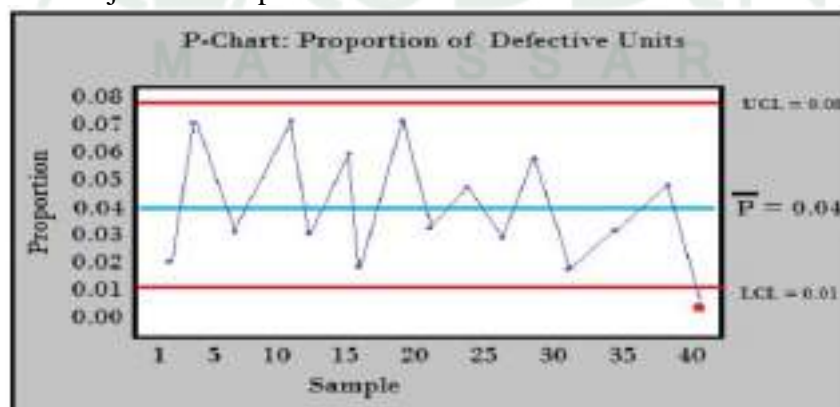
Gambar 2.5 :p-chart
