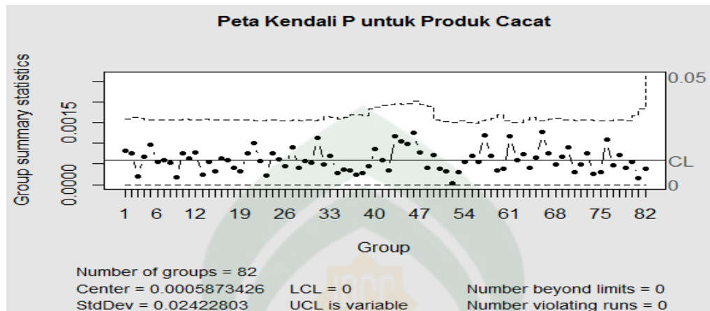
Gambar 4.1 p-chart PT. Makassar Tene
