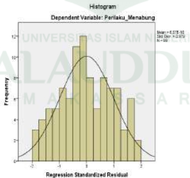
Gambar 4.2 Histogram
