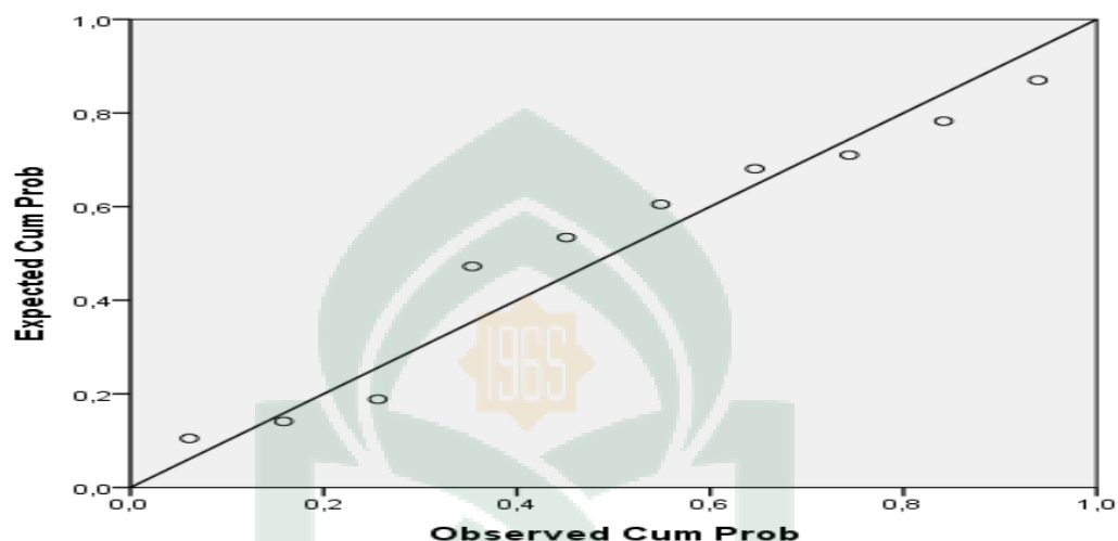
Gambar 4.1 Normal P-P Plot of Regression Standardized Residual Dependent Variable: Kemiskinan (Sumber: Output Olahan Data, 2018)
