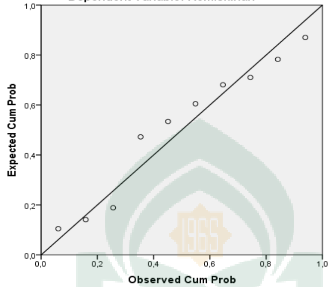
Normal P-P Plot of Regression Standardized Residual Dependent Variable: Kemiskinan
