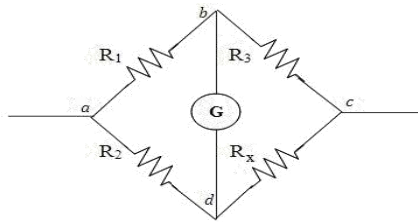
Gambar 1.1: Jembatan Wheatstone
