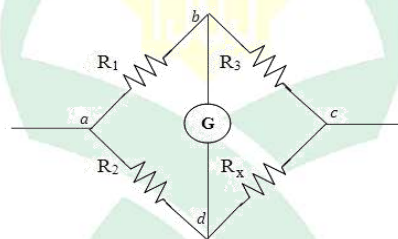
Gambar 1.1: Jembatan Wheatstone
