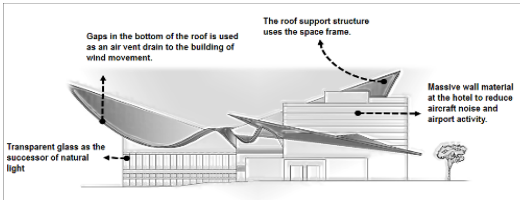
Fig. 9. Illustration of roof structure and building material
