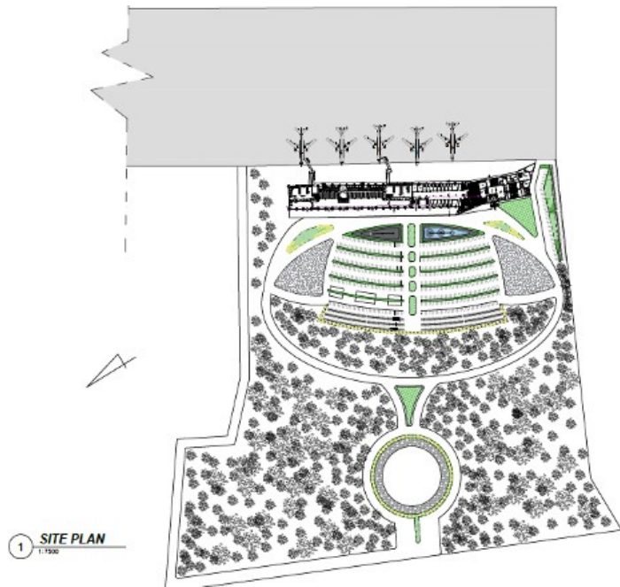
Fig. 6. Layout plan
