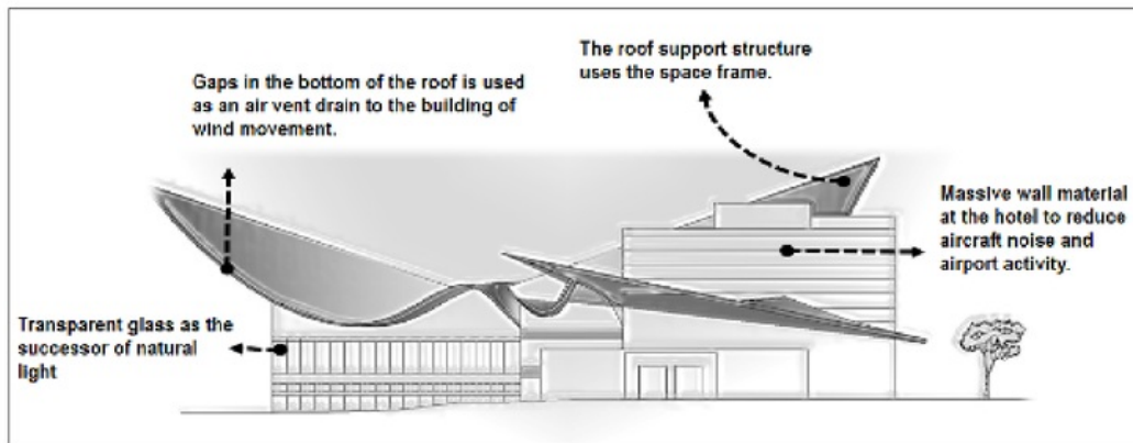
Fig. 9. Illustration of roof structure and building material
