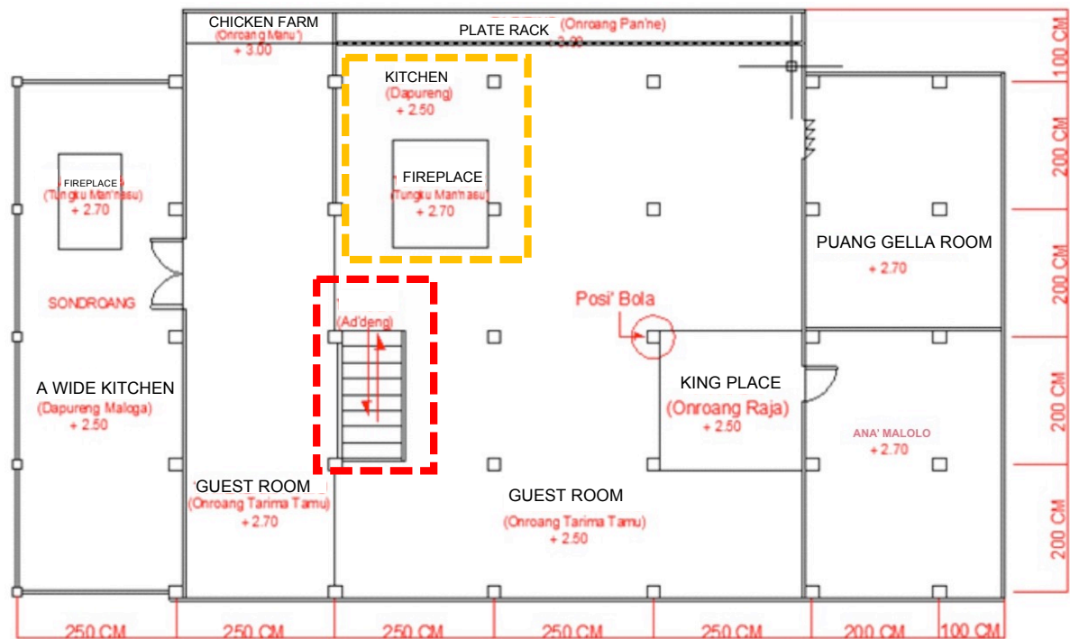
Figure 6 : Karampuang traditional house blueprint
