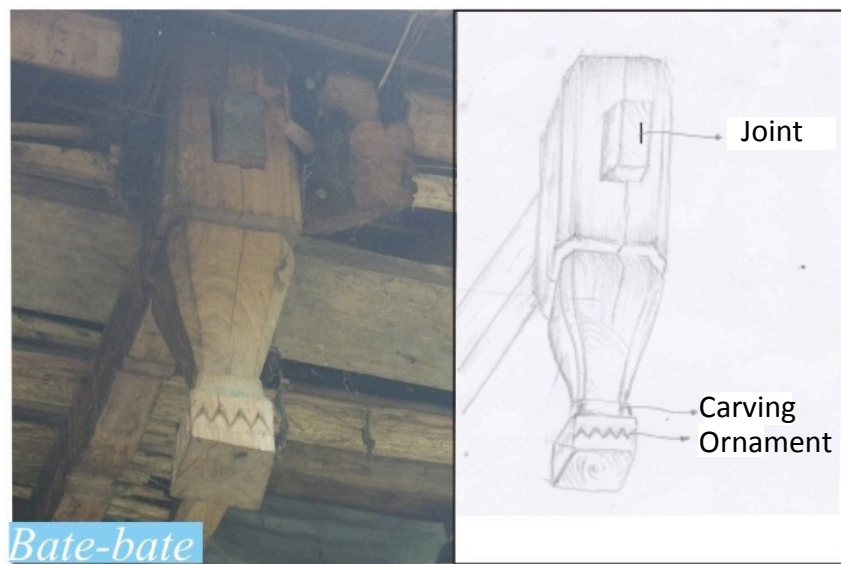
Figure 4 : Detail of bate-bate in Karampuang traditional house
