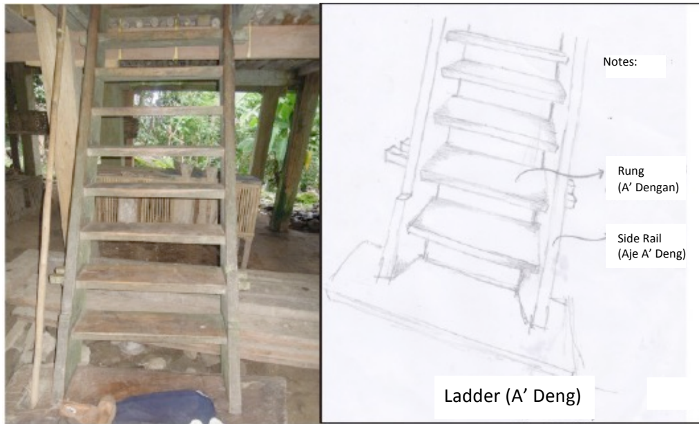
Figure 3 : Ladder detail for Karampuang traditional house
