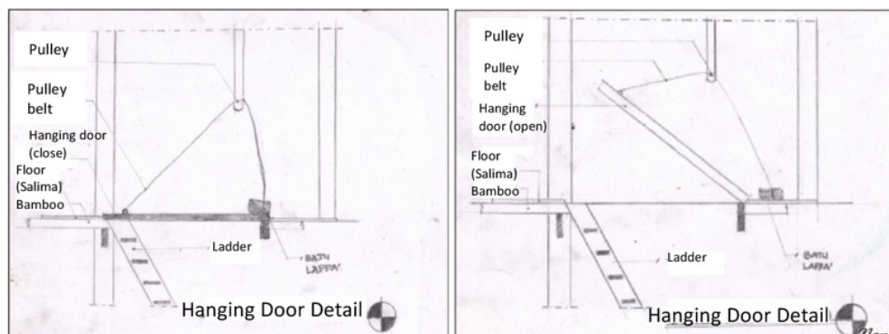
Figure 2: (a) Detail of the door in close condition; and (b) Detail of the door in open condition
