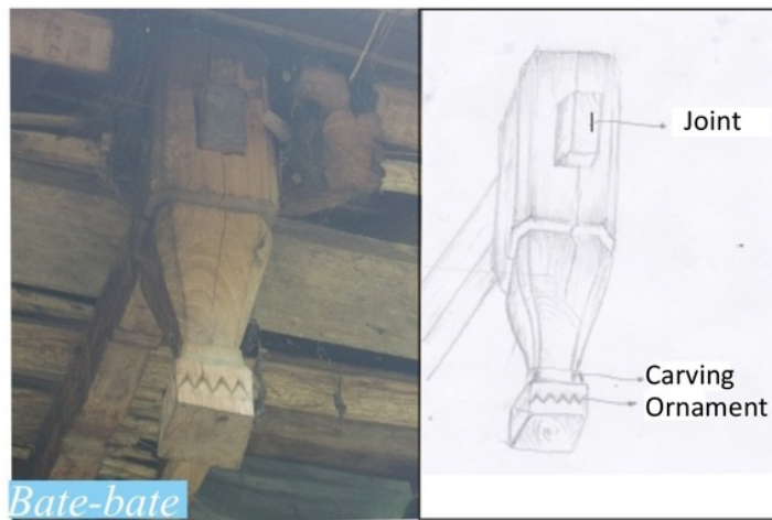
Figure 4 : Detail of bate-bate in Karampuang traditional house
