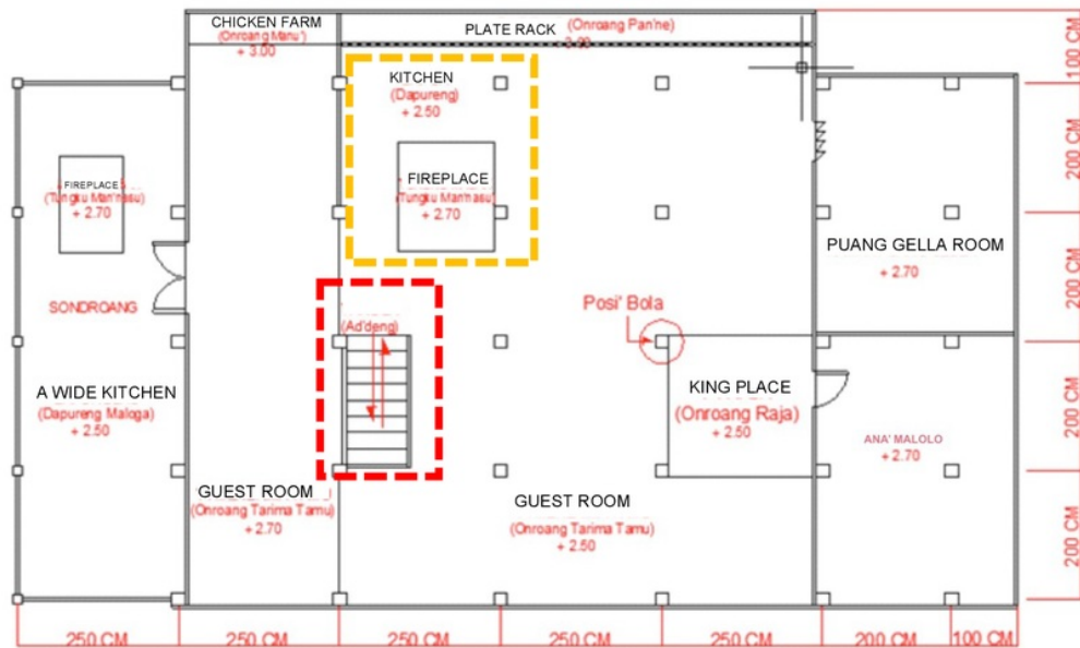
Figure 6 : Karampuang traditional house blueprint
