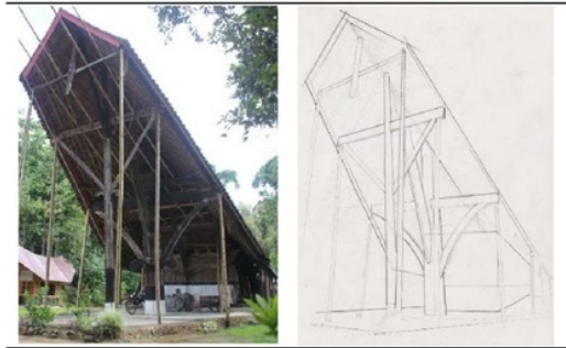
Fig. 5. Banua Layuk Roof Form
