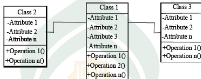
Gambar II. 4. Model Class diagram (Munawar, 2005).
