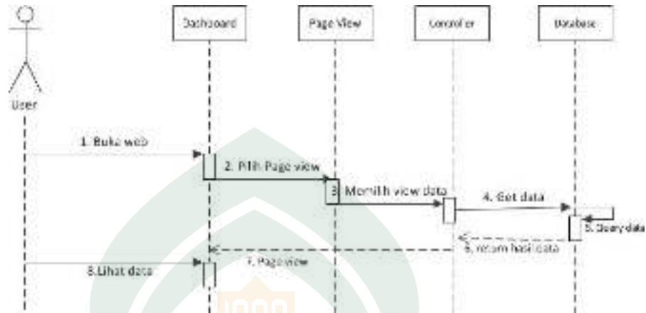
Gambar IV.6. Sequence diagram view data
