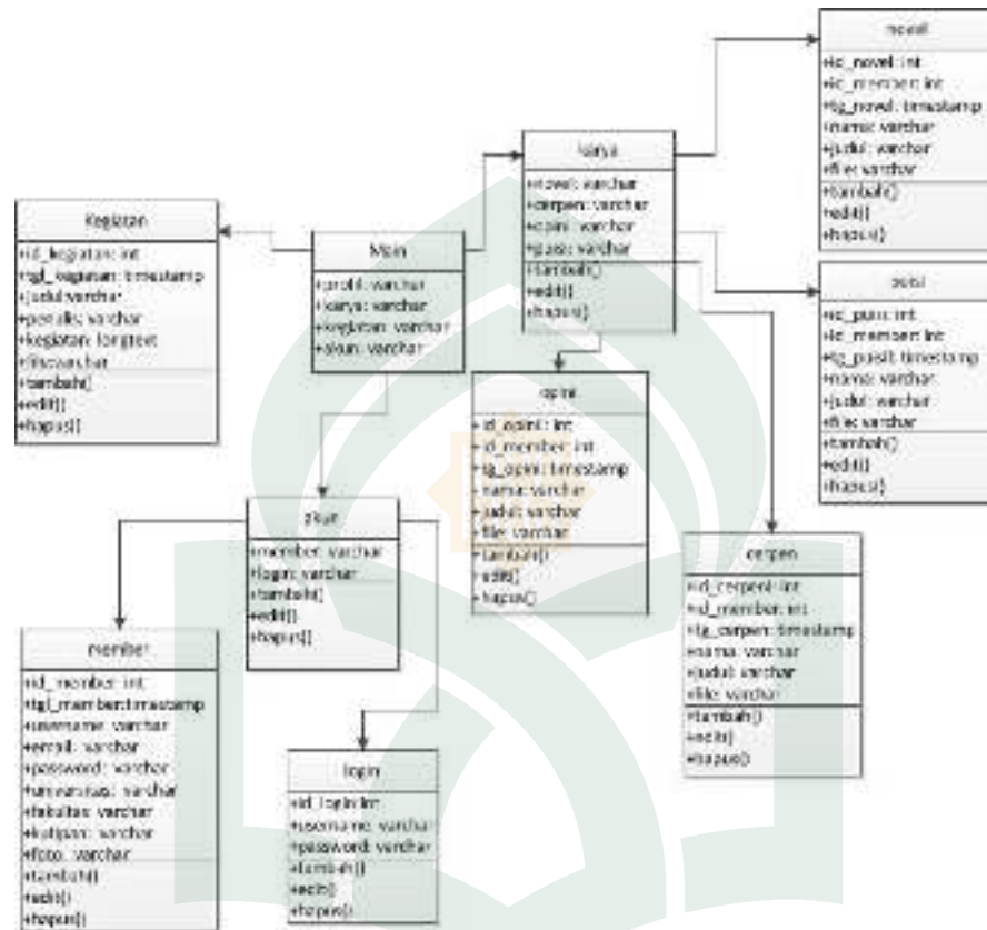
Gambar IV.11 Class diagram
