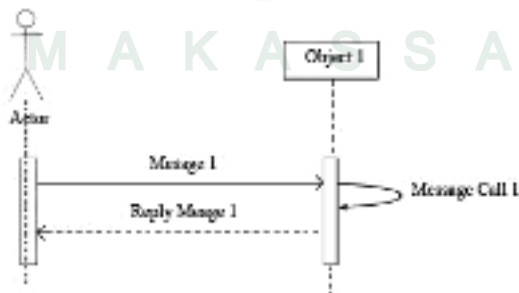
Gambar II. 2. Model Sequence Diagram (Munawar, 2005).
