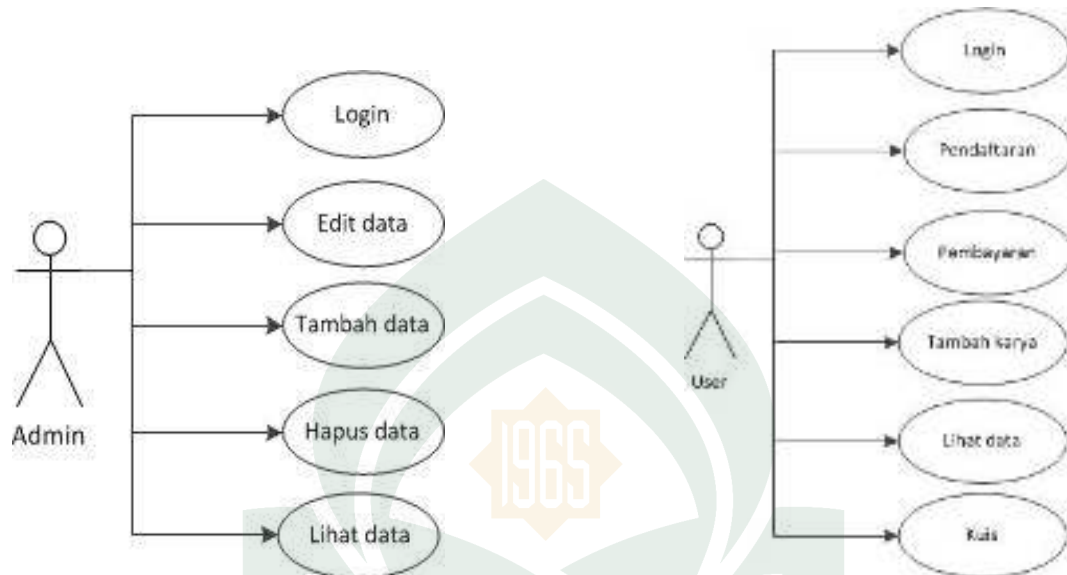
Gambar IV.4 Use case diagram
