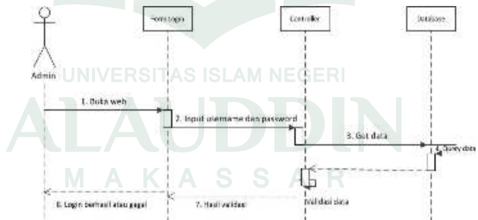
Gambar IV.5 Sequence diagram login
