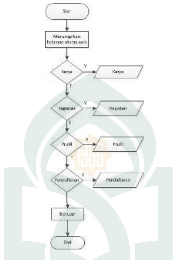
Gambar IV.3. Flowchart
