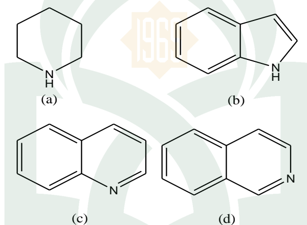
Gambar II.2: Kerangka dasar alkaloid
