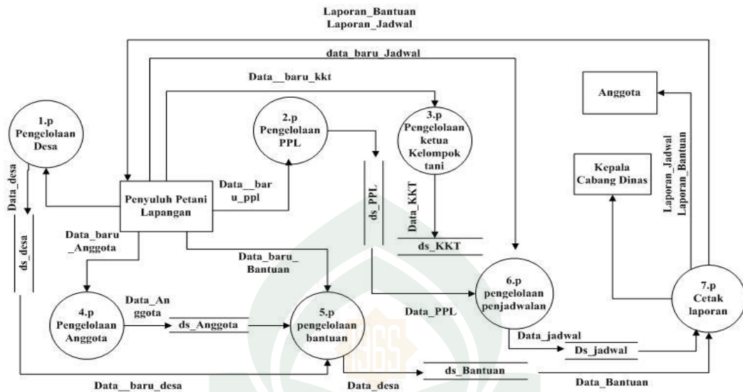
Gambar IV.5. Data Flow Diagram Level 1
