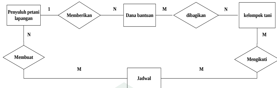
Gambar IV.7. Entity Relationship Diagram (ERD)
