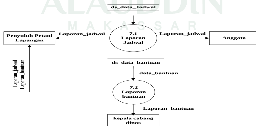
Gambar IV.6. Data Flow Diagram Level 2 Proses 7
