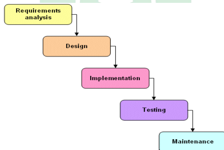
Gambar III. 1 Proses Waterfall(Nurasiah 2014)
