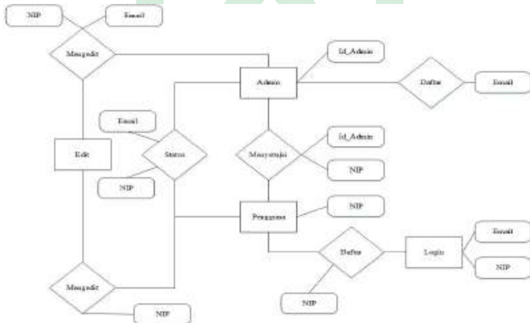
Gambar IV.24 Diagram Entitas
