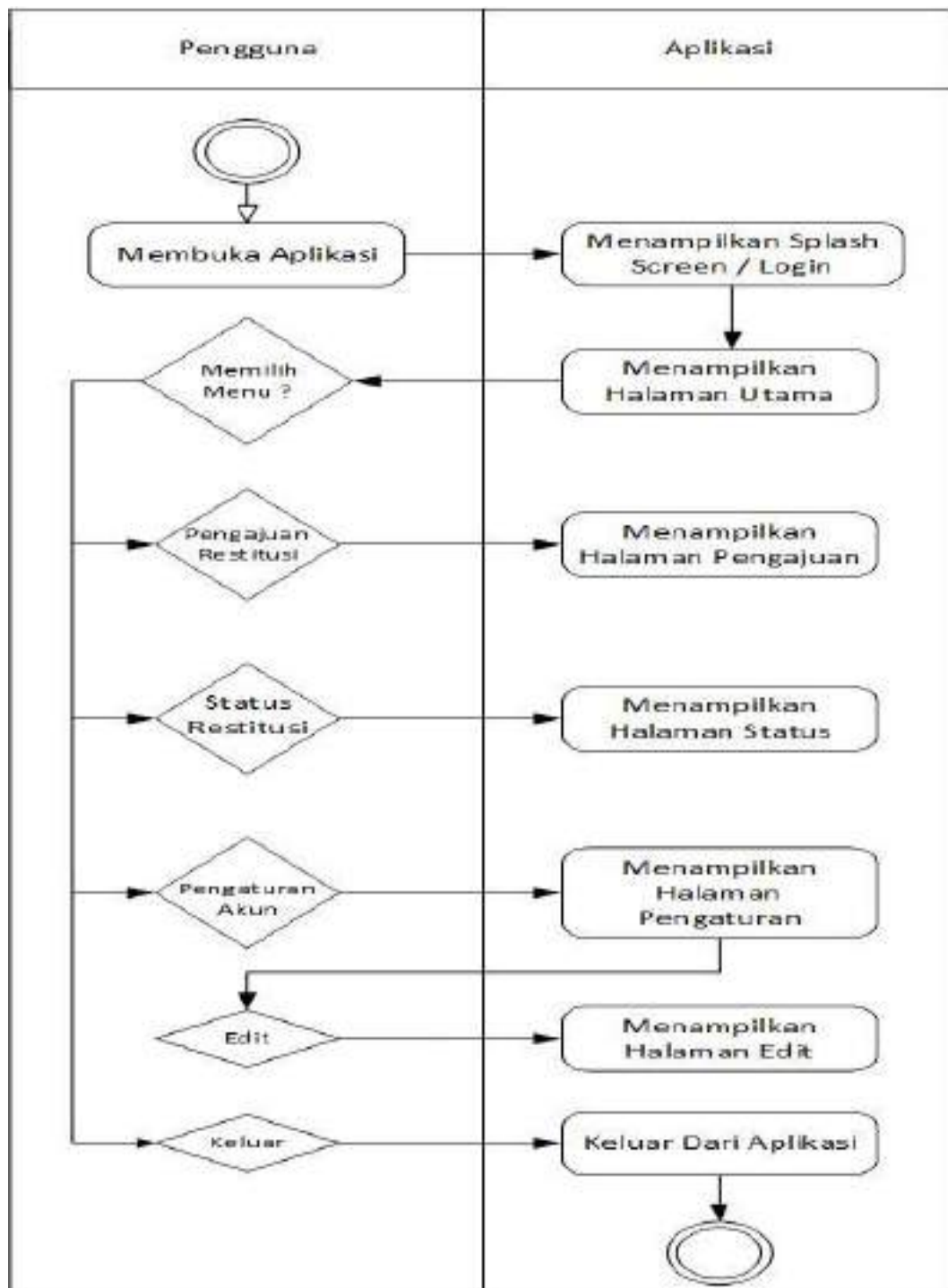
Gambar IV. 7 Activity diagram
