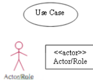
Gambar II.4. Simbol actor
