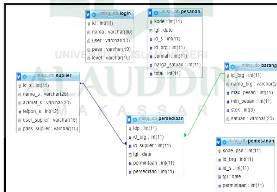
Gambar 4.11 Class Diagram
