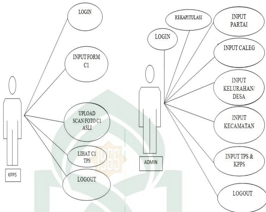
Gambar IV. 3 Use Case Diagram
