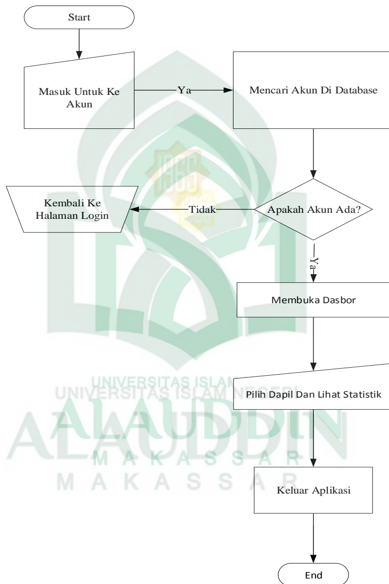
Gambar IV.8 Flowchart Sistem
