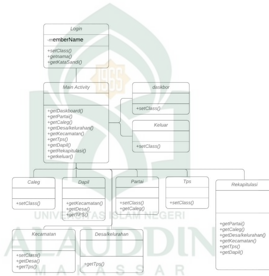
Gambar IV. 4 Class Diagram
