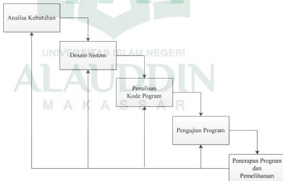
Gambar III.1 Metode waterfall
