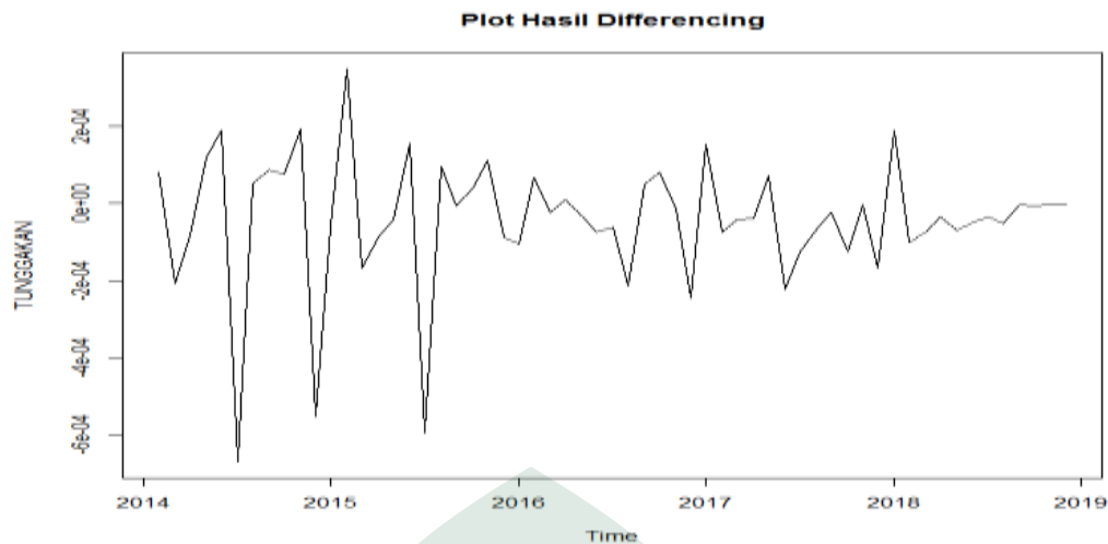
Gambar 4.7 Plot data setelah differencing
