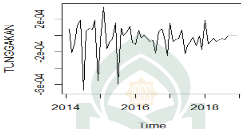
Plot Hasil Differencing
