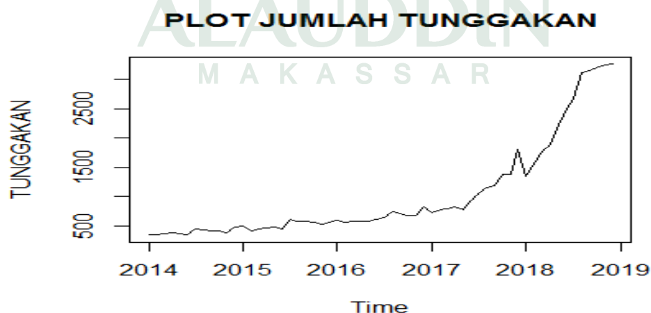
Gambar 4.3 plot time series data tunggakan
