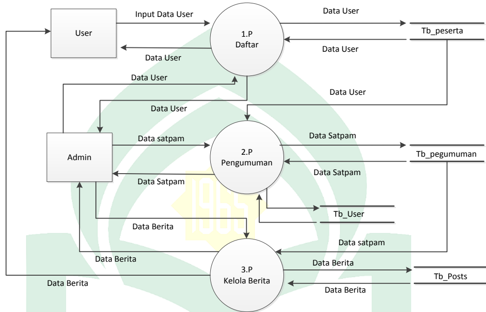
Gambar IV.5 Diagram Level 1
