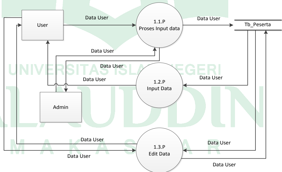
Gambar IV.6 Diagram Level 2 Proses 1
