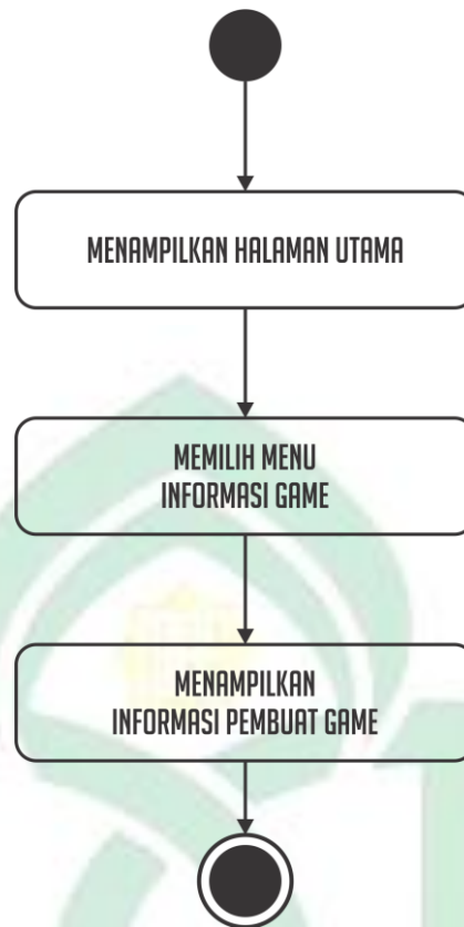
Gambar IV.8. Activity Diagram Informasi Game
