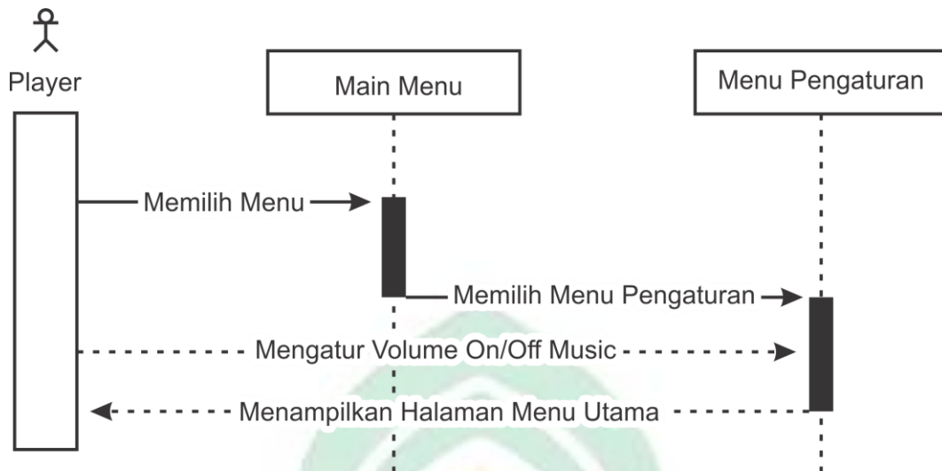
Gambar IV.13. Sequence Diagram Pengaturan
