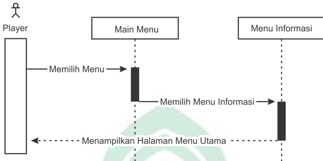
Gambar IV.14. Sequence Diagram Informasi Game
