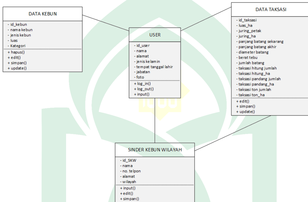
Gambar IV. 4 Class Diagram
