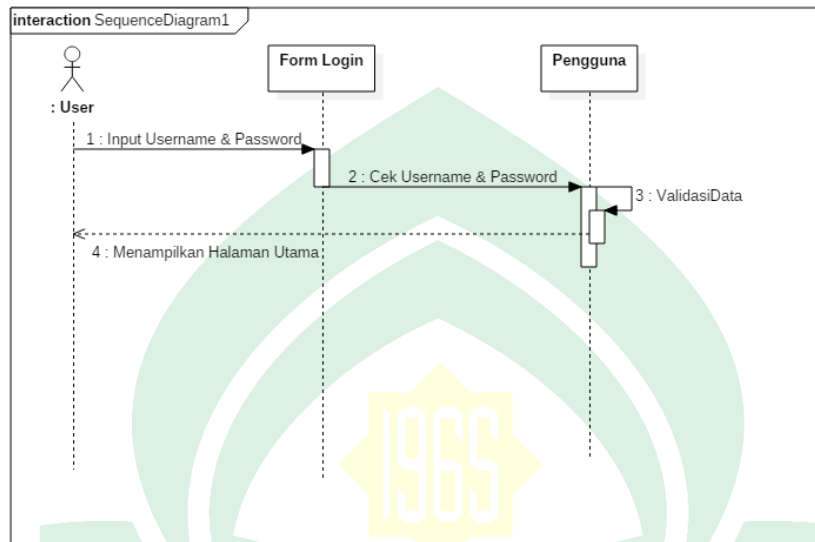
Gambar IV. 5 Sequence Diagram Login User
