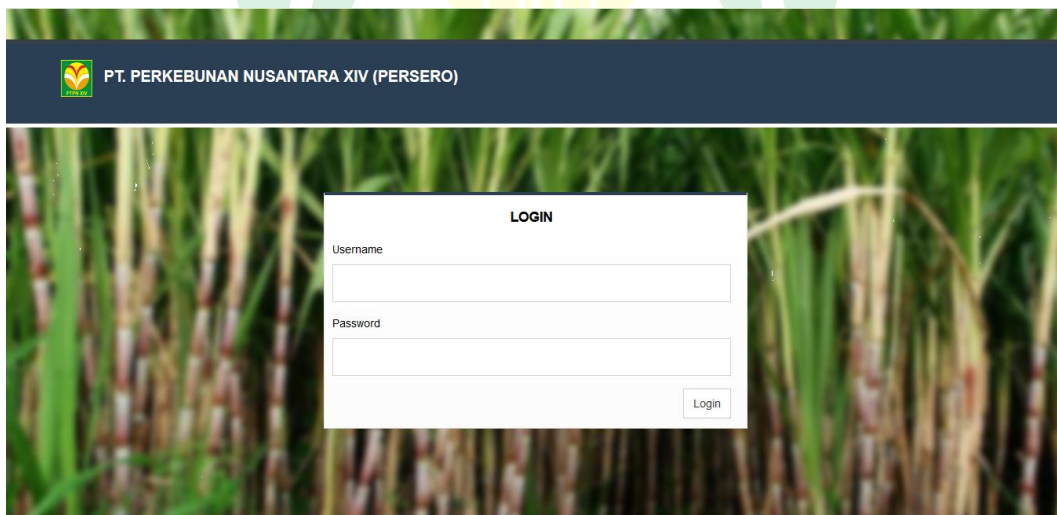
Gambar V. 1 Tampilan Login
