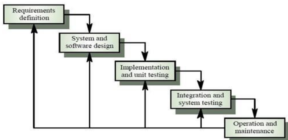
Gambar III .1. Model Waterfall
