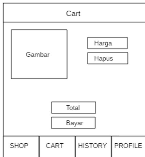
Gambar IV .16. Halaman Cart
