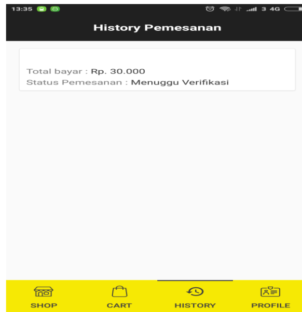
Gambar V.9. gambar History
