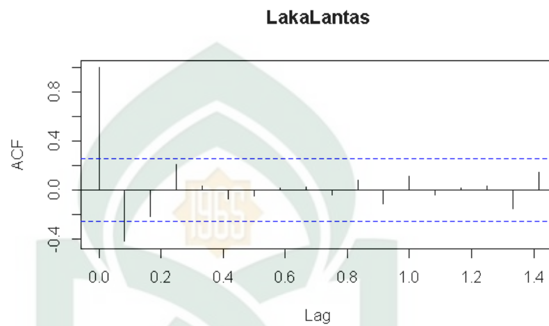
Gambar 4.7 Plot ACF Differencing Laka Lantas
