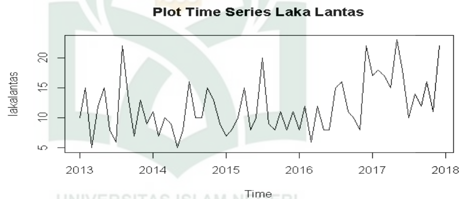
Gambar 4.1 Time Series Plot Jumlah Laka Lantas
