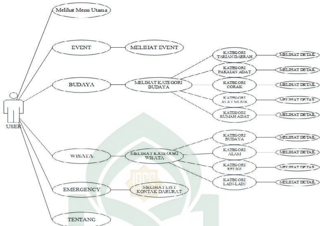
Gambar IV.3 Use Case Diagram
