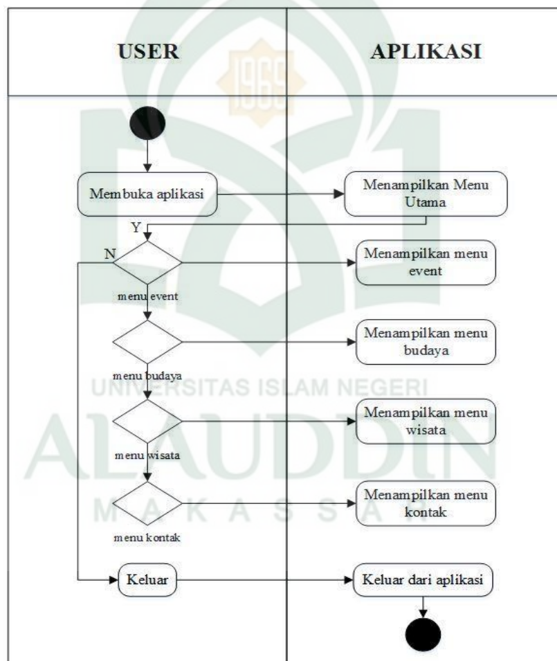
Gambar IV.11 Activity Diagram
