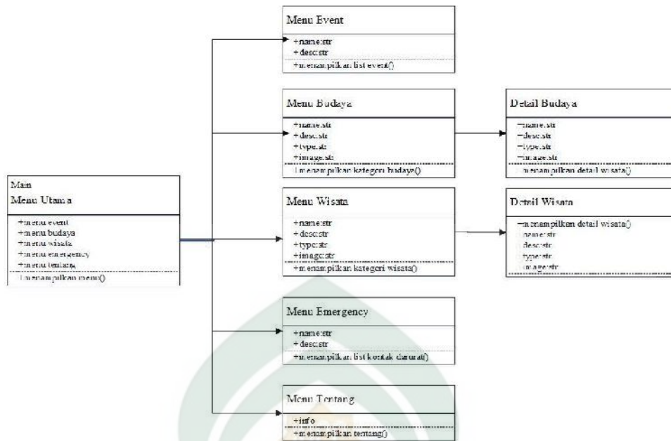
Gambar IV.4 Class Diagram
