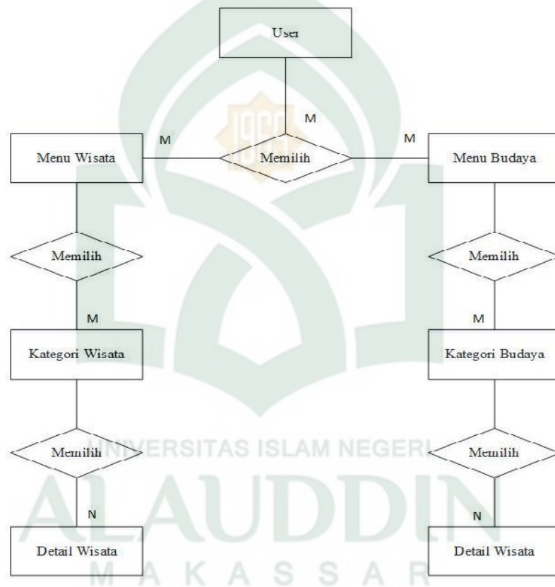
Gambar IV.12 Entity Relationship Diagram (ERD)
