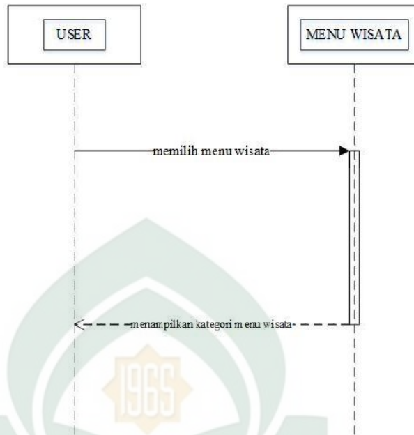
Gambar IV.9 Sequence Diagram menu wisata
