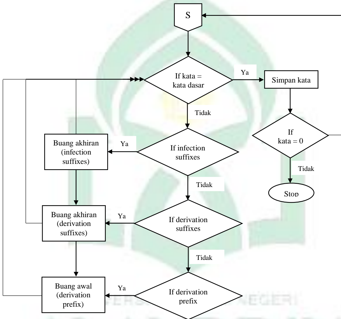
Gambar IV.8 Flowchart Steaming
