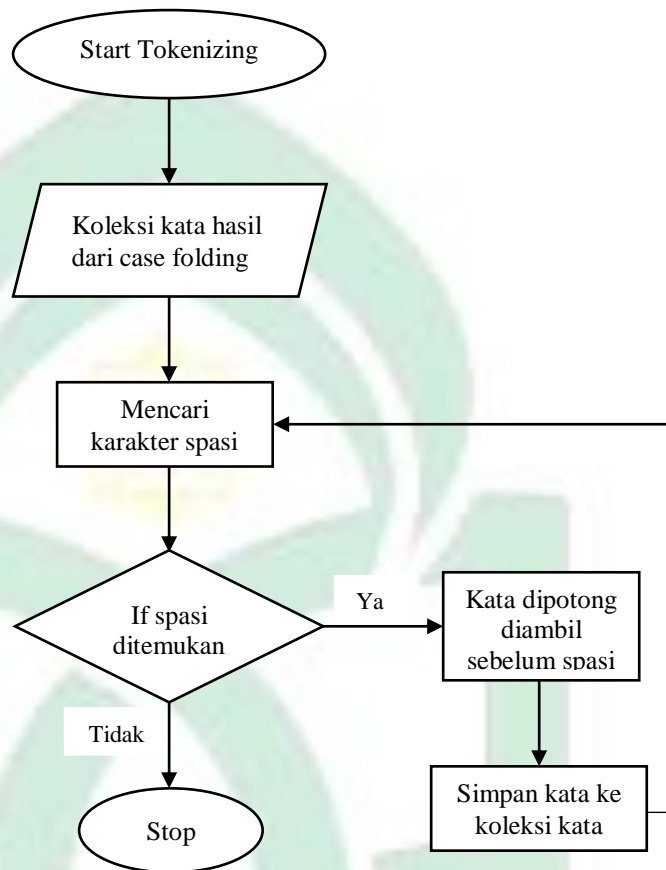
Gambar IV.6 Flowchart Tokenizing
