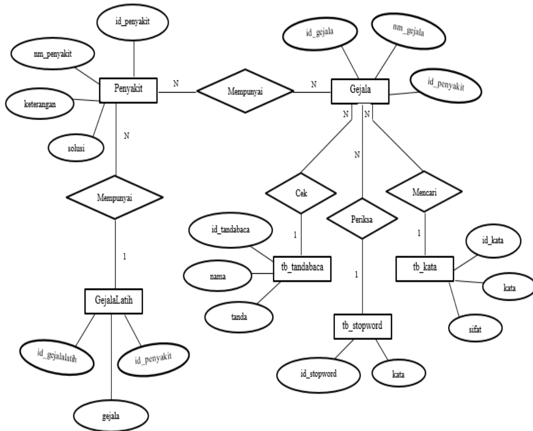
Gambar IV.12 Entity Relationship Diagram (ERD)
