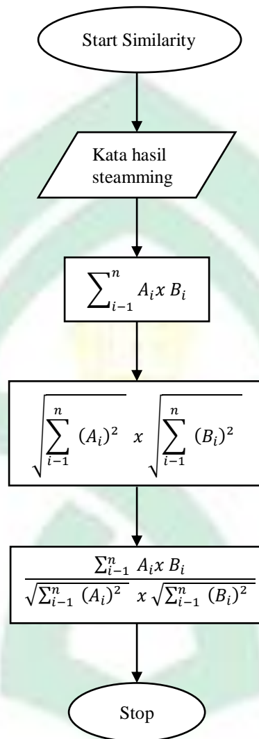
Gambar IV.9 Flowchart Cosine Similarity
