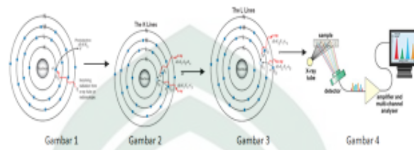
Gambar II. 6 X-ray Fluorescence (XRF)
