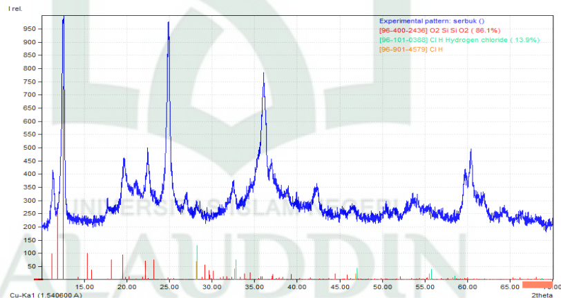
Gambar IV. 1 Hasil XRD Silika ( \text{SiO}_2 )
