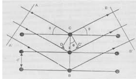
Gambar II. 5 Hukum Bragg
